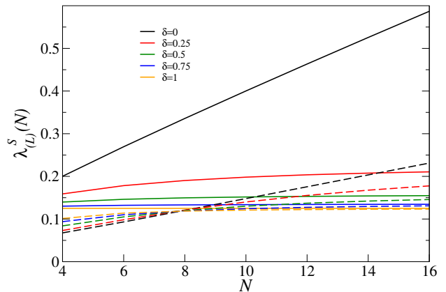
FIG. 5. The OBC spin localization tensor \lambda_{(L)}^S(N) (solid lines) and the PBC spin localization tensor \lambda_L^S(N) (dashed lines) as a function of the number of electrons N for various values of the dimerization parameter \delta in a Heisenberg model.
