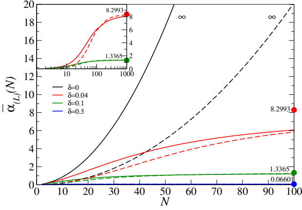
FIG. 2. The OBC polarizability \bar{\alpha}(N) (solid lines) and the PBC polarizability \bar{\alpha}_L(N) (dashed lines) as a function of the number of electrons N for various values of the dimerization parameter \delta in a tight-binding model. The dots and numbers next to each curve are the values of the PBC localization tensor in the thermodynamic limit. They were obtained from Eq. (24). Inset: \bar{\alpha}(N) and \bar{\alpha}_L(N) for \delta = 0.04 and \delta = 0.1 for large N .
