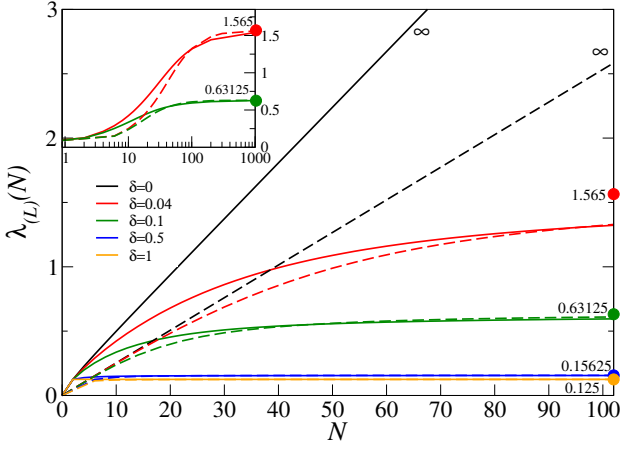
FIG. 1. The OBC localization tensor \lambda(N) (solid lines) and the PBC localization tensor \lambda_L(N) (dashed lines) as a function of the number of electrons N for various values of the dimerization parameter \delta in a tight-binding model (see Eqs. (16) and (17)). The dots and numbers next to each curve are the values of the PBC localization tensor in the thermodynamic limit. They were obtained from Eq. (22) with d = 1 . Inset: \lambda_L(N) for \delta = 0.04 and \delta = 0.1 for large N .
