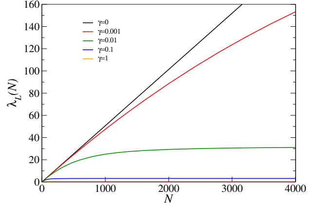
FIG. 3. The PBC localization tensor \lambda_L(N) as a function of the number of electrons N for various values of the electronegativity difference \gamma for a square lattice in a tight-binding model.
