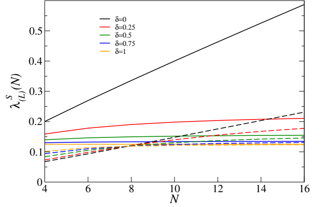
FIG. 5. The OBC spin localization tensor \lambda^S(N) (solid lines) and the PBC spin localization tensor \lambda_L^S(N) (dashed lines) as a function of the number of electrons N for various values of the dimerization parameter \delta in a Heisenberg model.
