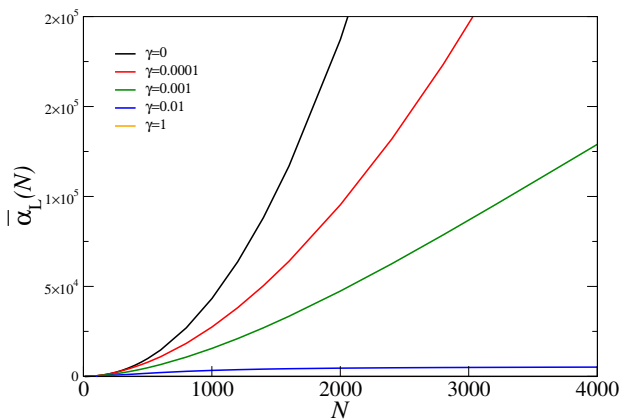
FIG. 4. The PBC polarisability \bar{\alpha}_L(N) as a function of the number of electrons N for various values of the electronegativity difference \gamma for a square lattice in a tight-binding model.
