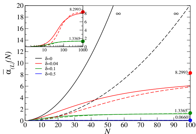
FIG. 2. The OBC polarizability \bar{\alpha}(N) (solid lines) and the PBC polarizability \bar{\alpha}_L(N) (dashed lines) as a function of the number of electrons N for various values of the dimerization parameter \delta in a tight-binding model. The dots and numbers next to each curve are the values of the PBC localization tensor in the thermodynamic limit. They were obtained from Eq. (24). Inset: \bar{\alpha}(N) and \bar{\alpha}_L(N) for \delta = 0.04 and \delta = 0.1 for large N .
