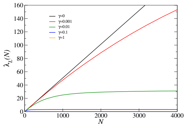
FIG. 3. The PBC localization tensor \lambda_L(N) as a function of the number of electrons N for various values of the electronegativity difference \gamma for a square lattice in a tight-binding model.
