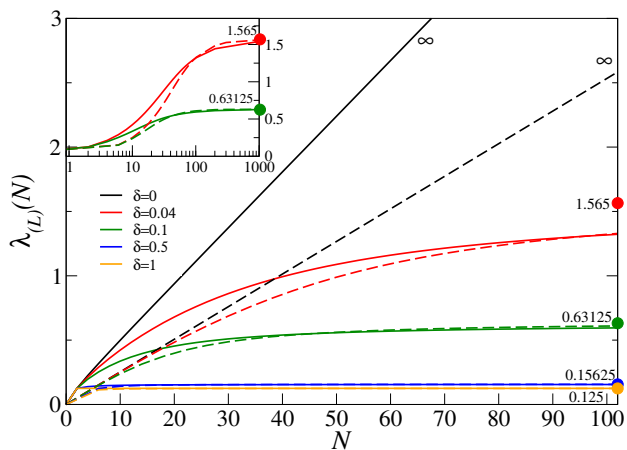
FIG. 1. The OBC localization tensor \lambda(N) (solid lines) and the PBC localization tensor \lambda_L(N) (dashed lines) as a function of the number of electrons N for various values of the dimerization parameter \delta in a tight-binding model (see Eqs. (16) and (17)). The dots and numbers next to each curve are the values of the PBC localization tensor in the thermodynamic limit. They were obtained from Eq. (22) with d = 1 . Inset: \lambda_L(N) for \delta = 0.04 and \delta = 0.1 for large N .
