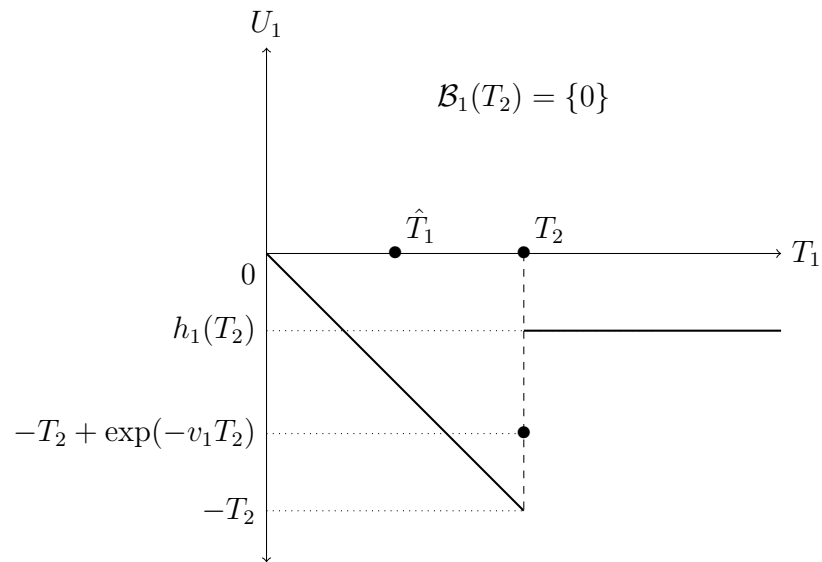
Figure A.5: Case (b) T_2 > \hat{T}_1
