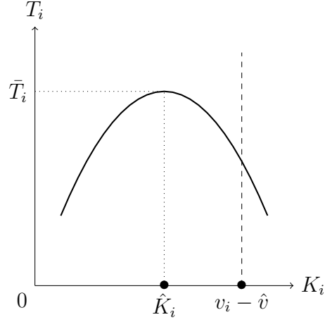
Figure 3: overestimation effect - v_i \in [v, \bar{v}]
