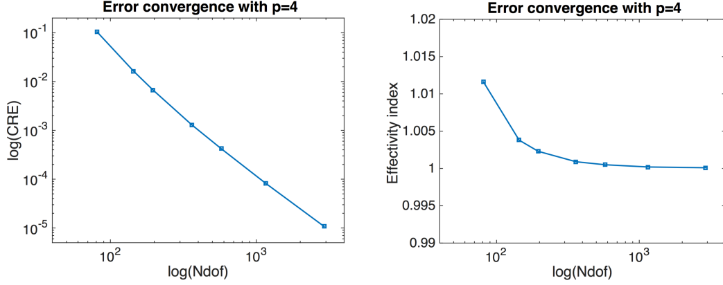
Figure 32: Convergence of the CRE estimate (left) and the global effectivity index (right) with respect to the number of dofs for p = 4 .
