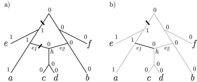
FIGURE 1. a) The hardwired parsimony score of the depicted network is 2, while the softwired parsimony score is 1 (one of the possible trees displayed by the network is depicted in gray in b). Changes are depicted by thick lines crossing the branches.
