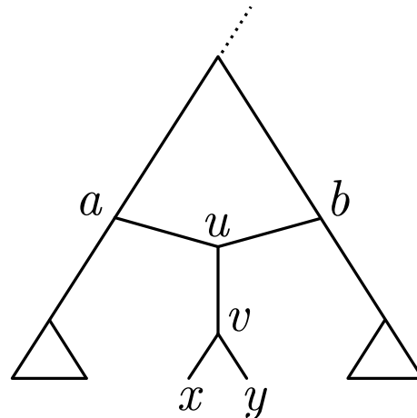
FIGURE 8. The gadget used in the NP-hardness proof.
