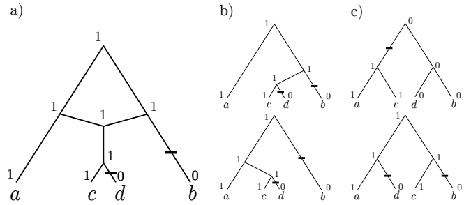
FIGURE 7. The different parsimony scores of the network N given in Figure 5 are 2, 2 and 1 for the hardwired, softwired and parental parsimony, respectively: a) An optimal extension for the hardwired PS; b) Optimal extensions for the two trees displayed by N for the softwired PS; c) Optimal extensions for the two other parental trees of N (the ones that are not depicted in b)) for the parental PS. Changes are depicted by a thick line.
