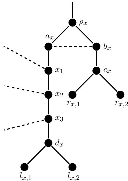
FIGURE A1. Example gadget G_x . Solid edges are in E_= , dashed edges are in E_\neq . Nodes x_1, x_2, x_3 represent three copies of the vertex x , with incident dashed edges going to nodes corresponding to the three neighbors of x . Leaves are assigned as follows: g'(r_{x,1}) = g'(l_{x,1}) = 1 , g'(r_{x,2}) = g'(l_{x,2}) = 2 . The gadget enforces that x_1, x_2, x_3 must all be assigned the same value.
