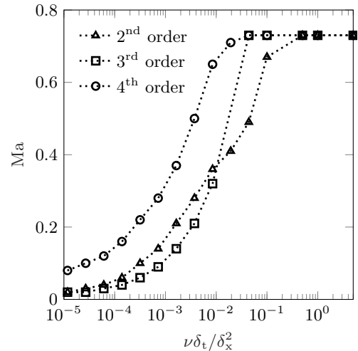
FIG. 1: Effects of the EDF order on the linear stability domain of the SRT collision model.
