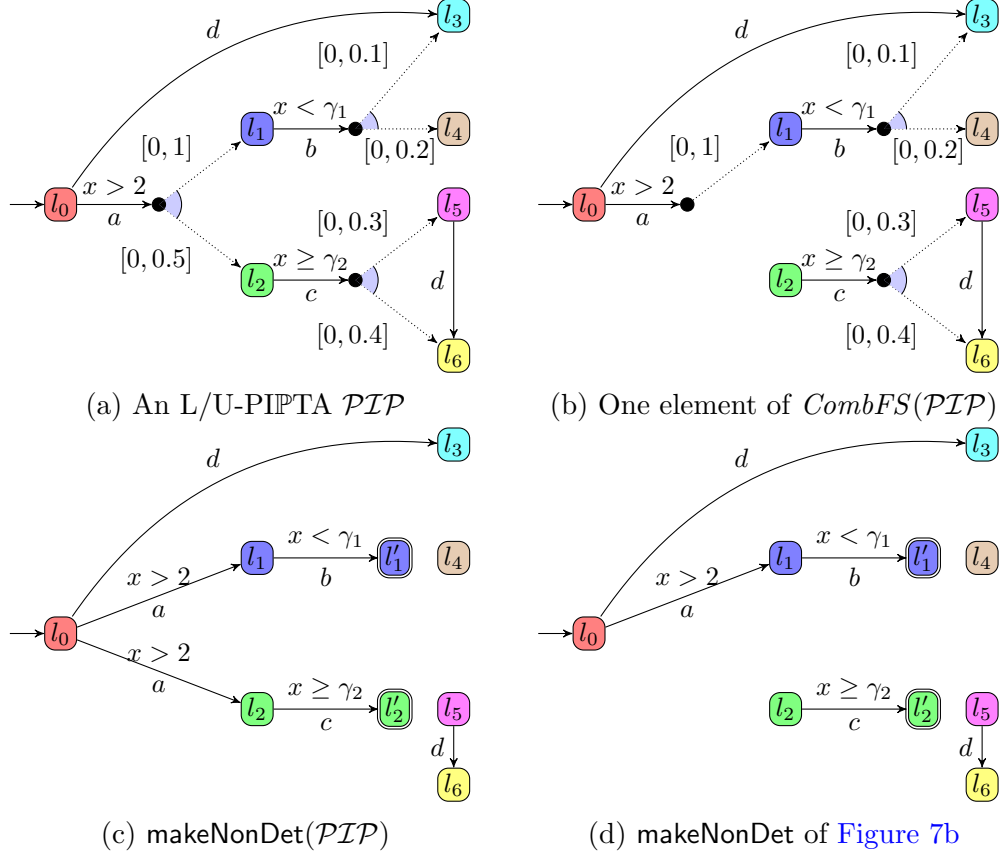
Figure 7: Exemplifying \text{CombFS} , \text{makeNonDet} and \text{makeAcc}
