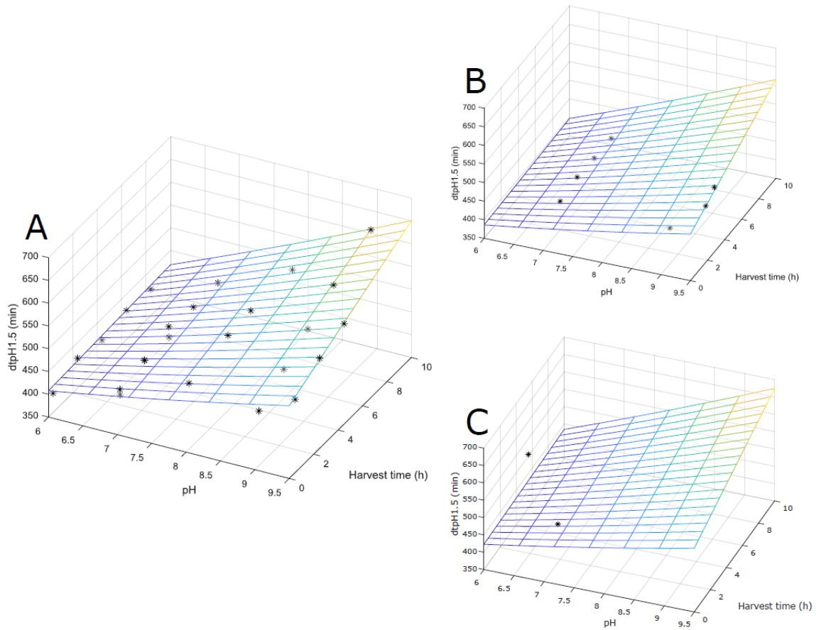
Figure 3: Response surface representations of the effect of fermentation pH and harvest time on the dtpH1.5 values of C. maltaromaticum CNCM I-3298 concentrates produced at 30 °C (A) , 20 °C (B) and 37 °C (C) . *experimental data points employed in the model at the given temperatures.
