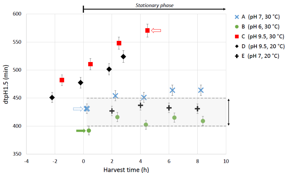
Figure 4: \text{dtpH1.5} values of C. maltaromaticum CNCM I-3298 concentrates harvested at increasing times of fermentation, carried out at different values of pH and temperature. Fermentation conditions leading to best (full green arrow) and worst (empty red arrow) acidification activities are indicated, as well as the reference conditions corresponding to the TopCryo® commercial TTI (dashed, empty blue arrow). The range of acidification activities leading to technologically similar shelf-lives to the control is signaled by dotted lines. Harvests done before stationary phase are of no industrial interest.
