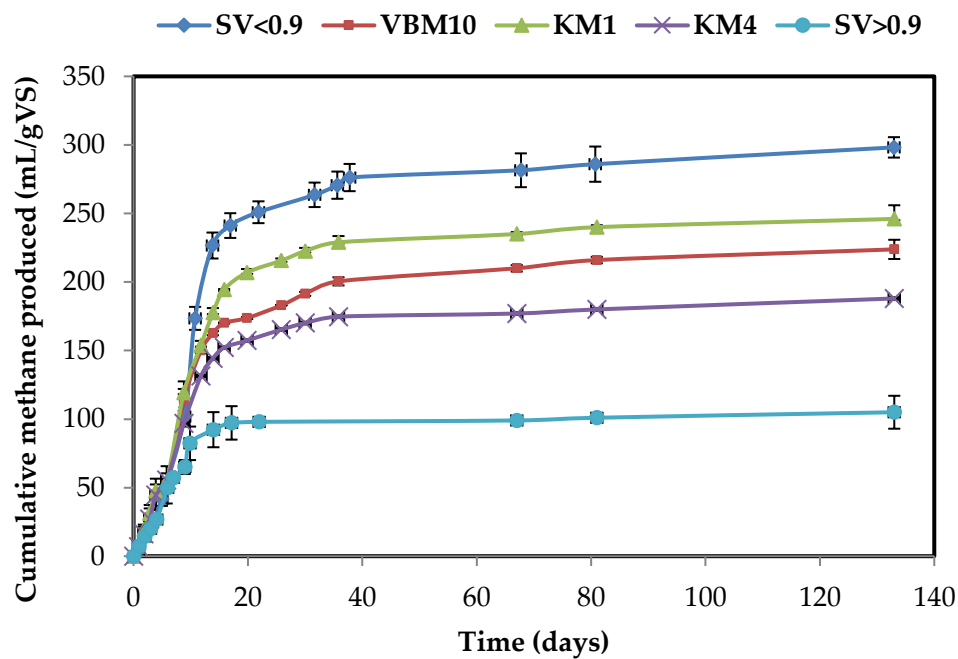
Figure 4. Cumulative methane production for different dry fractionation process of T olive pomace from three-phase extraction process: (A) Milling pretreatments and (B) dry separation process (electrostatic and sieving).
