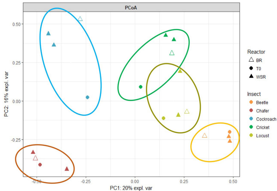
FIGURE 5 | Principal coordinate analysis (PCoA) plot showing similarity relationships among bacterial community sampled from three groups of insect bioreactors (36% of the total variance explained).
