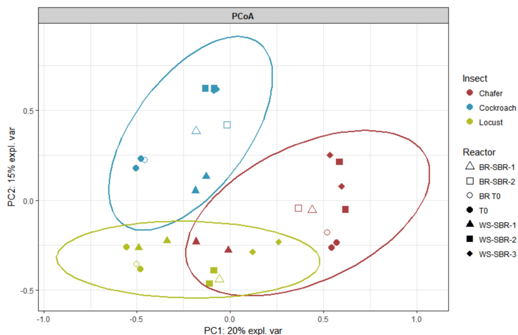
FIGURE 9 | Principal coordinate analysis (PCoA) plot showing similarity relationships bacterial communities present within insect gut microbiomes before (T0) and at the end (WS-SBR and B-SBR) of cultures in successive batch reactors maintained at pH8. PCoA was conducted given the Hellinger distance matrix.
