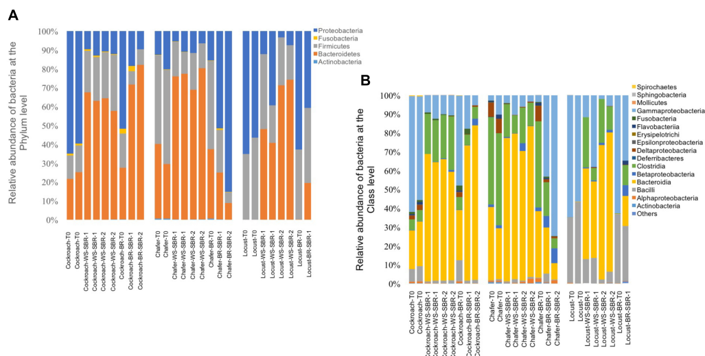
FIGURE 8 | Relative abundance of bacteria phylum (A) and bacteria class (B) identified from the Illumina Miseq sequencing data, within insect gut microbiomes before (T0) and after cultures in successive batch reactors maintained at pH8: duplicate WS-SBR-1 and WS-SR-2 were fed with wheat straw and BR-SBR contained insect gut without wheat straw among two successive batch.
