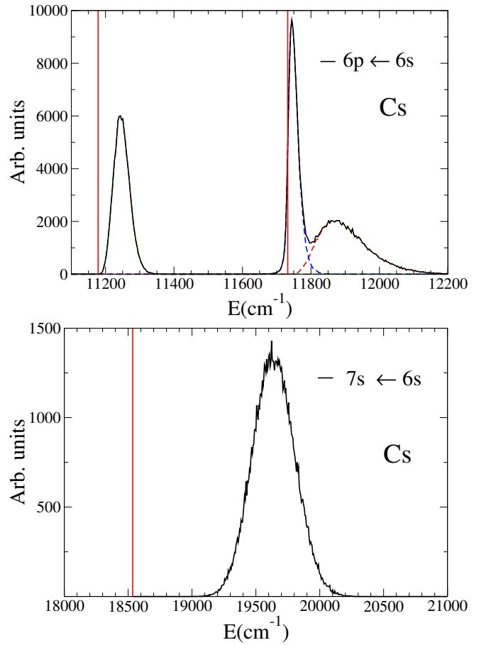
Fig. 2. Top: Dipole absorption spectrum of Cs@ 4 He 1000 around the 6p \leftarrow 6s transition (arbitrary units). The vertical thin lines represent the free Cs atom transitions; the low energy D1 line comes entirely from excitation to the ^2\Pi_{1/2} state. The high energy D2 line is decomposed into its ^2\Pi_{3/2} (blue dashed line) and ^2\Sigma_{1/2} (red dotted line) components. Bottom: same as top for the 7s \leftarrow 6s transition.
