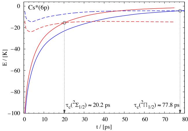
Fig. 5. U^+(t) for Cs in the 6p\ ^2\Sigma_{1/2} and 2\Pi_{1/2} states (solid lines). Also shown are the \text{Cs}^* kinetic energies of Fig. 3 changed of sign (dashed lines). The intersection of the U^+(t) and -E_{kin}(t) curves corresponding to the same state yields the fall-back time \tau_c [Eq. (12)] for that state.
