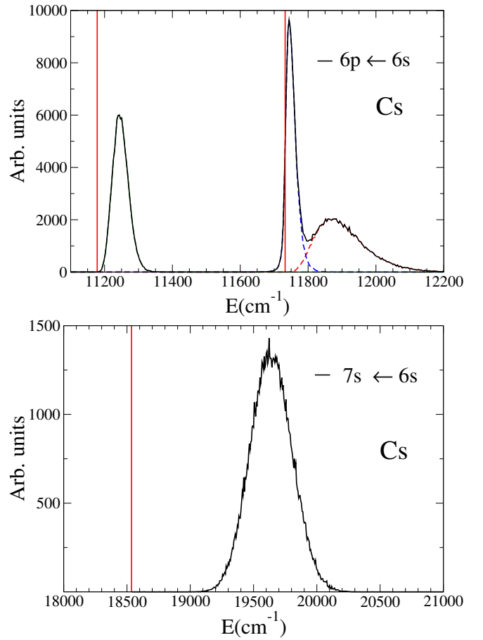
Fig. 2. Top: Dipole absorption spectrum of \text{Cs}@^4\text{He}_{1000} around the 6p \leftarrow 6s transition (arbitrary units). The vertical thin lines represent the free Cs atom transitions; the low energy D1 line comes entirely from excitation to the ^2\Pi_{1/2} state. The high energy D2 line is decomposed into its ^2\Pi_{3/2} (blue dashed line) and ^2\Sigma_{1/2} (red dotted line) components. Bottom: same as top for the 7s \leftarrow 6s transition.
