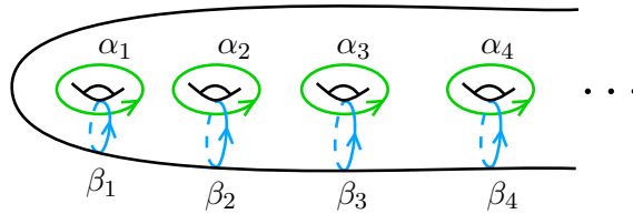
FIGURE 8. A geometric basis for the Loch Ness monster surface
