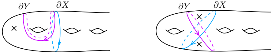
FIGURE 3. Two pairs of flare surfaces with the same homology, but different spaces of ends
