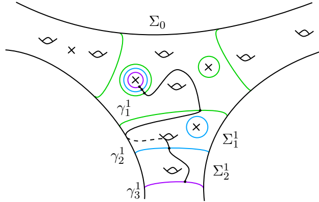
FIGURE 11. An example of the sequence of subsurfaces constructed in the proof of Proposition A.8
