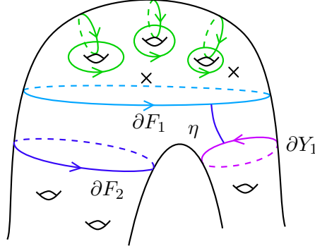
FIGURE 6. Constructing the Y_j
