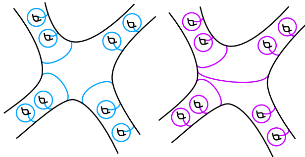
FIGURE 10. Two geometric symplectic bases that are not in the same mapping class group orbit.
