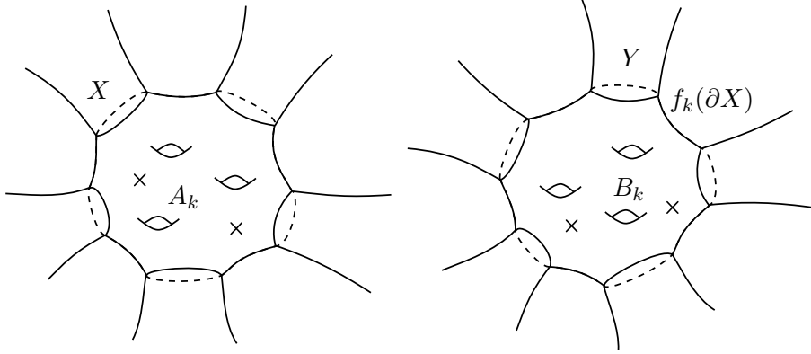
FIGURE 5. The subsurfaces in condition (4)
