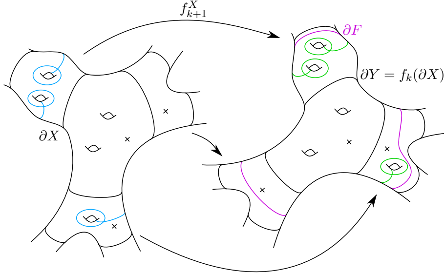
FIGURE 7. From k to k + 1 in the proof of Theorem 2
