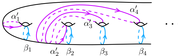
FIGURE 9. Curves representing the same basis as the curves in Figure 8
