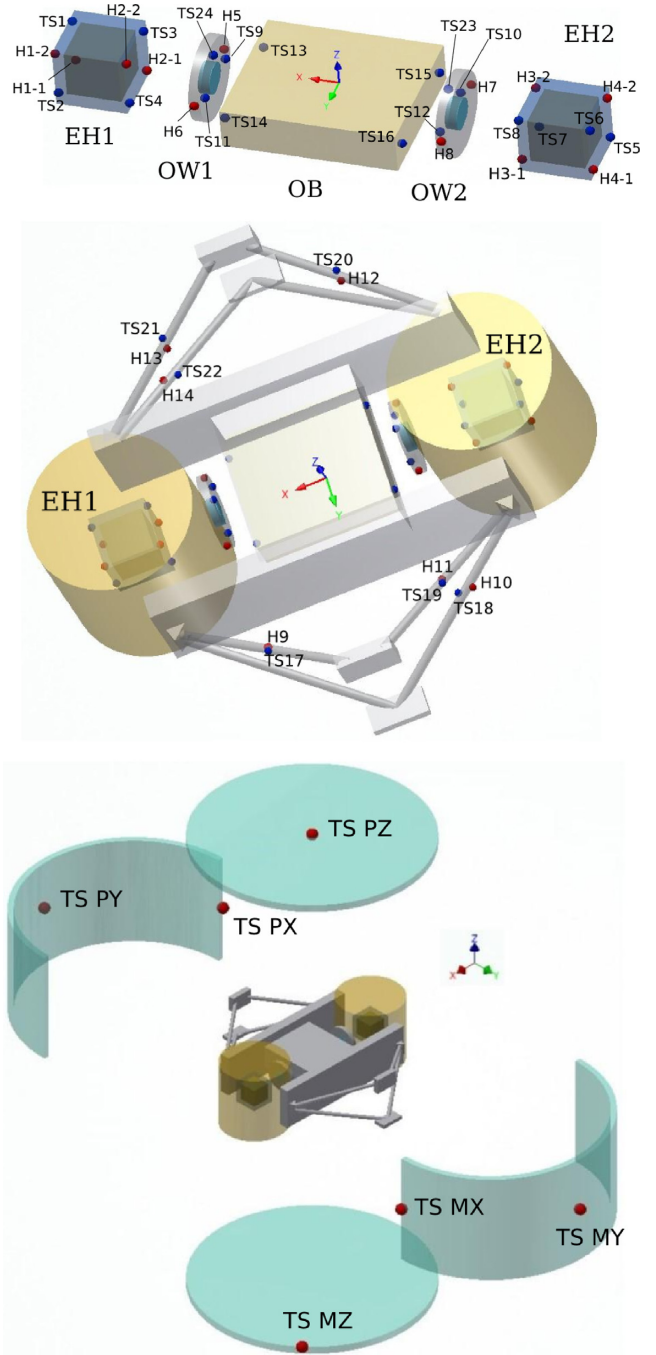
Figure 1. Distribution of temperature sensors in LPF. Top: Heaters and temperature sensors in the electrode housing (EH), the optical window (OW), and the optical bench (OB) from the diagnostics subsystems. Middle: Temperature sensors and heaters in the struts from the diagnostics subsystems. Bottom: Some of the platform sensors attached to thermal shield surrounding the instrument.
