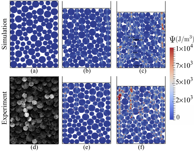
FIG. 7. Snapshots of the uniaxial compression of an assembly of elastic cylinders for the numerical simulations (a–c) with \mu_f = 0.3 and the experiments (d–f). The packing fractions of the systems are \Phi = 0.78 (a, d), \Phi = 0.83 (b, e), \Phi = 0.88 (c, f). Snapshot (d) shows the initial positions of particles in the experimental setup. The strain energy density \Psi represented with the same color code in panels (a)–(c) and (e) and (f).
