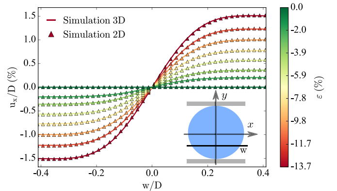
FIG. 3. Dimensionless displacement field along the x direction u_x/D as a function of the Lagrangian transverse position w shown in inset, for several values of \varepsilon . Solid lines show the 3D numerical results with \nu = 0.495 (almost incompressible neo-Hookean material), whereas the triangles show the 2D numerical results with \nu = 1/3 .
