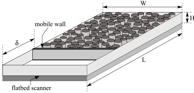
FIG. 1. Sketch of the experimental setup: a bidisperse assembly of cylindrical particles (diameters D_1 = 20 mm and D_2 = 30 mm, height H ) made of silicone rubber lays on a flatbed scanner. The system is compressed step by step by a mobile wall. The lower face of the cylinders is captured by the scanner. Dimensions of the setup are L = 286 mm, W = 202 mm, and H = 15 mm.
