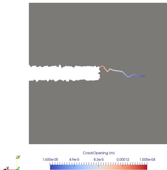
Figure 11: Crack pattern obtained with the second approach
