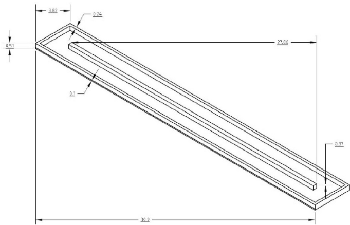
Fig. 1. The semi-buried raceway used for microalgal culture in Qatar.
