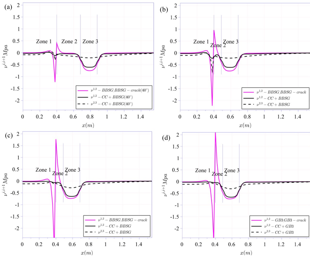
FIG. 3 - Interfacial normal stress comparison between the various cases: (a) BBSG (40°, E^3 = 1000\text{MPa} , w=0 ); (b) BBSG (40°, w=-0.2 ); (c) BBSG (15°C, w=-0.2 ) ; GB3 (15°C, w=-0.2 )
