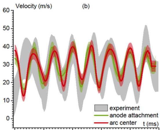
Fig. 6 Arc root velocity (7690 Hz, 5 mm)
