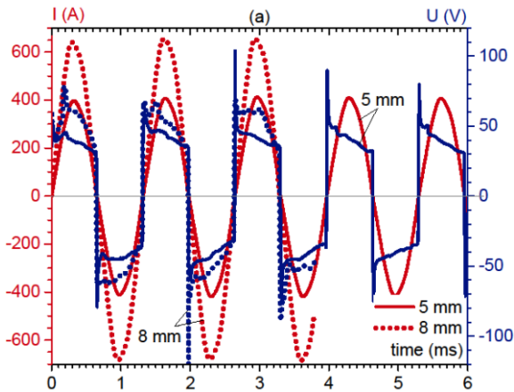
Fig. 3 Current and arc voltage (760Hz, h=5&8mm)
