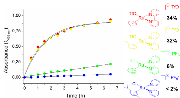
Figure 2. UV-vis monitoring (Abs @ \lambda = 459 nm) of the reaction between [(\eta^6\text{-arene})\text{Ru}(\text{bpy})\text{L}](\text{PF}_6) (arene = benzene or p -cymene; L = Cl or OTf) and 2 equivalents of 4,4'- (\text{CH}_2\text{PO}_3\text{Et}_2)_2\text{-bpy} ligand in refluxing ethanol. Right: Conversions in RuP 4 OEt -bpy calculated from the absorbance.
