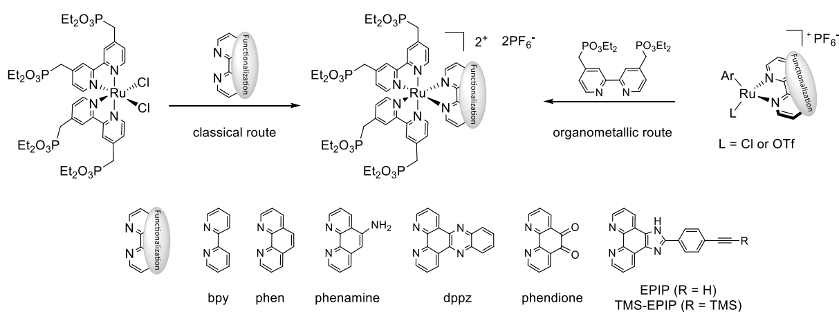
Figure 1. Schematic representation of the two synthetic routes to access the \text{RuP}_4^{\text{OEt}}\text{-N}^{\wedge}\text{N} complexes and structure of the \text{N}^{\wedge}\text{N} ligands employed in this study.
