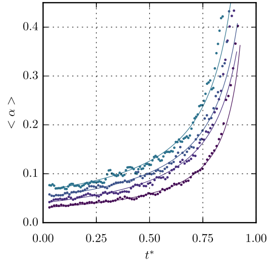
Fig. 14. Assessment of the space-averaged air volume prediction (8) for the four smallest d^* displayed in Fig. 13. The solid lines and dots refer to \langle \alpha \rangle_m and \langle \alpha \rangle , respectively.
