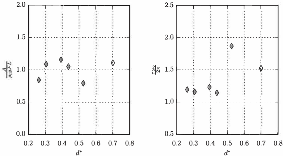
Fig. 16. Variation of the normalized amplitude \frac{A}{\rho_l g \mathcal{F} L} of pressure oscillations (left), and decay time \frac{\tau \omega_2}{2\pi} of the pressure transient (right), with respect to the normalized neck diameter d^* .
