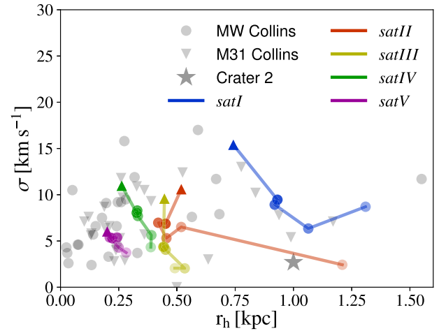
Figure 9. Projected velocity dispersion inside the stellar 2D half-mass radius as a function of the stellar 2D half-mass radius. Coloured triangles denote the isolated simulations while the filled circles denote the different orbits. The more violent the orbit, the fainter is the colour of the dots. Observations of Milky Way and M31 satellites (for references see Section 3.2) are shown as grey dots (and a star for the recently discovered satellite Crater 2) and triangles, respectively.
