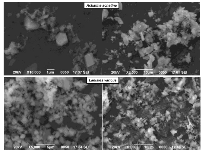
Figure 7. SEM images of synthesized bioceramics using microwave irradiation method
