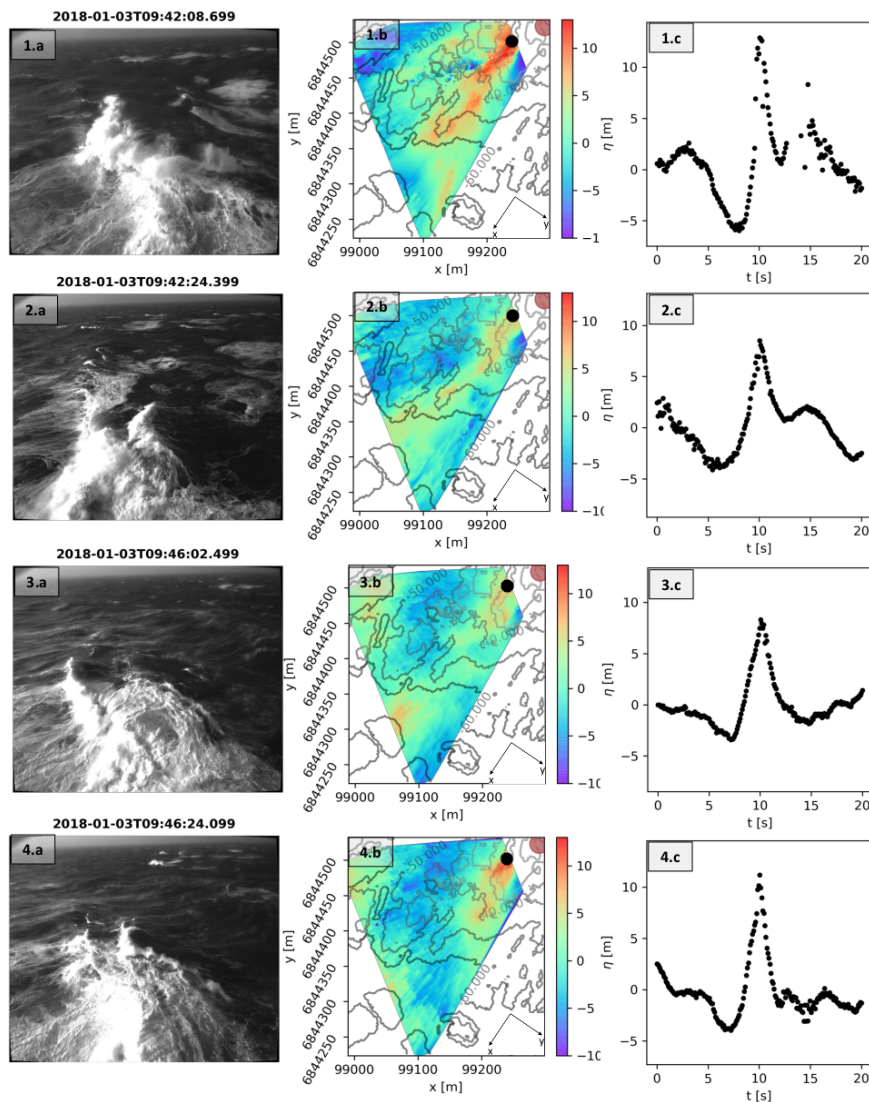
Figure 7. Description of the 8 high waves selected for our study (4 in this Figure and 4 in figure 8). Left panels: video images, middle panel reconstructed wave surfaces projected in a Lambert93 geographic system overlaid over iso-contours of water depths (the black dots show the extraction point of the time series analysed in the paper) right panels: time series of the high waves elevation, collected at x=99250\text{m} , y=6844500\text{m} from the stereo video reconstruction.
