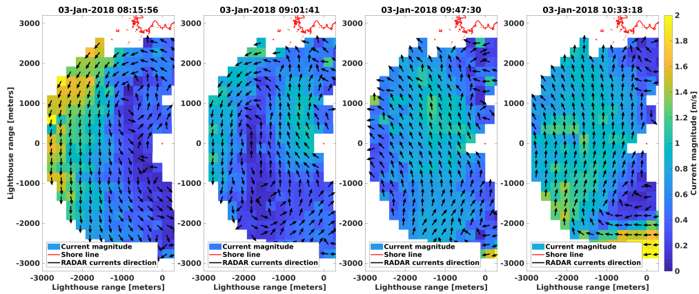
Figure 3. Marine radar retrieved current maps of January 3, 2018 between 0815 and 1030 UTC (left to right). The color coding gives the current magnitude and the unit vectors represent the current directions. Each map was generated from 15 minutes of marine radar data.
