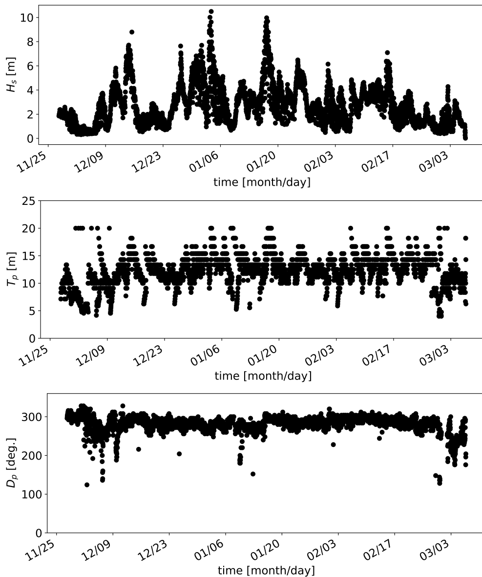
Figure 4. Time series of the significant wave height H_s , peak period, T_p and peak wave direction, D_p measured by the offshore wave buoy moored during winter 2017-18.
