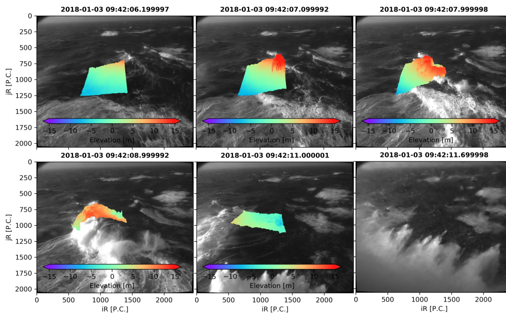
Figure 6. Examples of stereo video 3D surface elevation map z(iR, jR, t) plot over its corresponding right camera bitmap image in the pixel reference system. The colorbar shows the sea surface elevation and ranges from -15m (blue) to +15m (red) above the Mean Sea Level computed at the time of the record. The sequence of images shows an extreme breaking event (referred to as wave1 in the paper, corresponding wave height: 19.0 m). The reconstruction area was reduced in this illustration to highlights the breaking areas.
