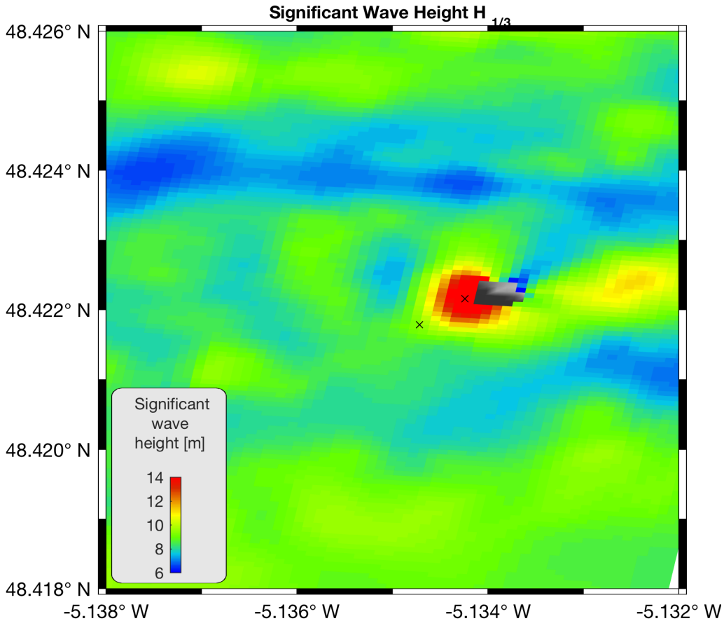
Figure 10. Significant wave height map obtained from the BOSZ model for the simulation corresponding to the wave event of 09:39 am on January 3.
