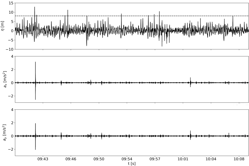
Figure 5. First panel, 30 min elevation time series for January 3 2019 (starting at 09:39:38 UTC) extracted from point ( X=99250\text{m}, Y=6844500\text{m} ) in the stereo images of Figures 7 and 8, the horizontal dashed line show the 8 m-elevation threshold used to select the individual waves studied in the paper. Second and third panel: accelerations along x and y axes for the same record measured by the highest accelerometer in the tower. The signal noise was filtered out using a Butterworth filter with a cut-off frequency of 50 Hz
