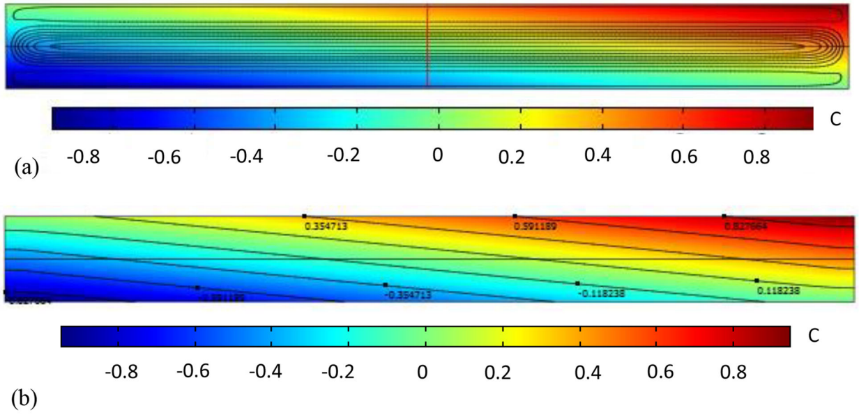
Fig. 9. Streamlines (a) and iso-mass fraction lines (b) obtained for A = 60 , Ra = -200 .
