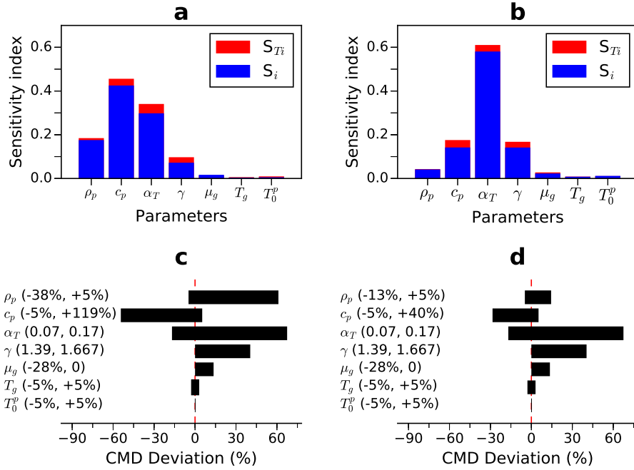
Fig. 3 The first-order S_i and the total-order S_{T_i} Sobol sensitivity index of the main parameters in the LII model at the Fe/C mass ratio (a) 1:1 and (b) 5:1. Uncertainties in particle sizing by LII at the Fe/C mass ratio (c) 1:1 and (d) 5:1.
