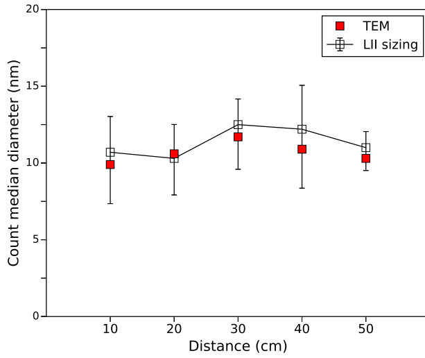
Fig. 5 NP size evolution in the gas phase at different positions in the CVD reactor at 850 °C.
