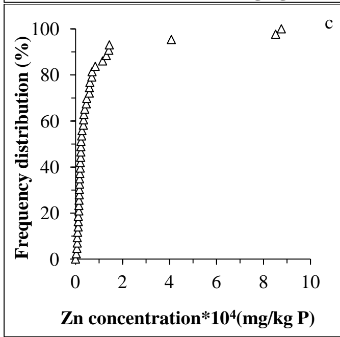
Figure 6. Frequency distribution of Cd (a), Pb (b), Zn (c) and Cu (d)
