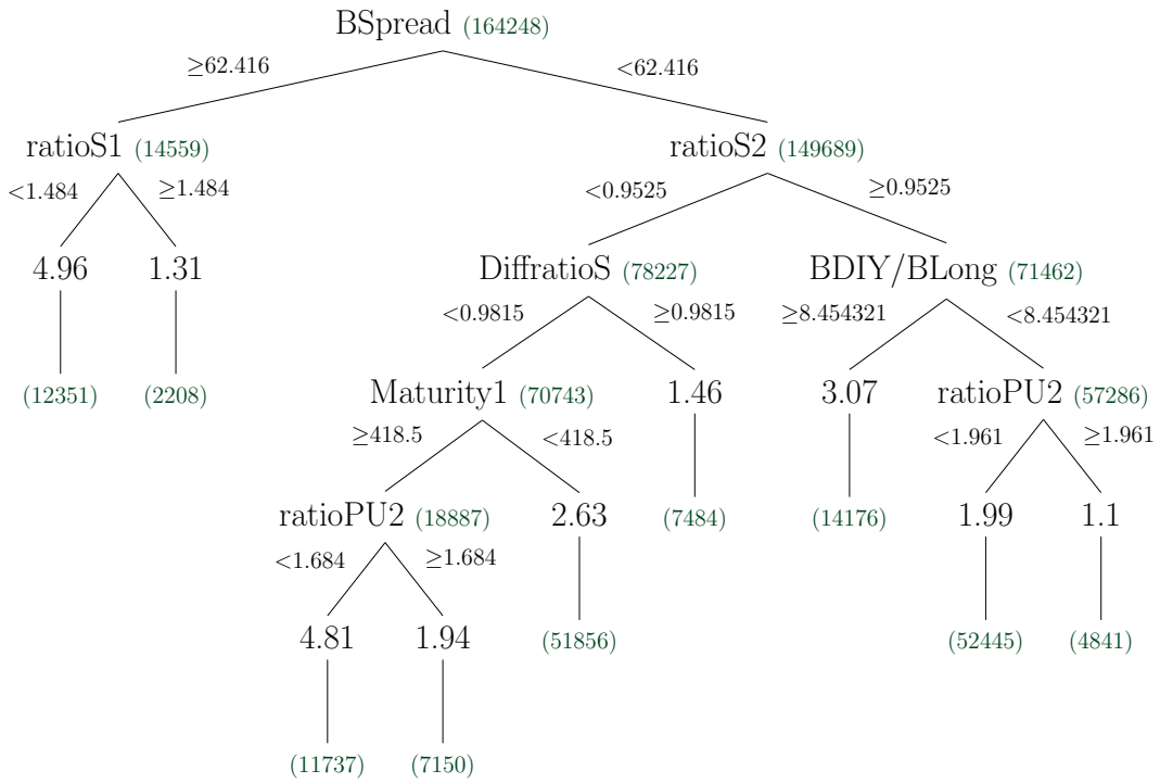
Figure 7: Second sub-tree
