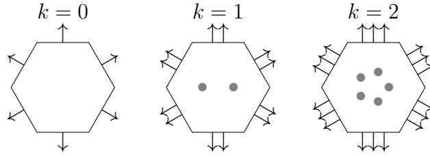
Fig. 5.8: Discrete unknowns in \underline{\Sigma}_T^k for k \in \{0, 1, 2\} .
