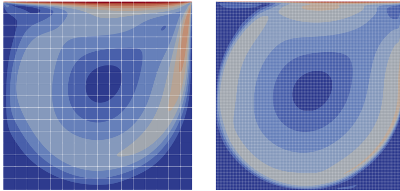
Fig. 9.1: Lid-driven cavity flow, velocity magnitude contours (10 equispaced values in the range [0, 1] ) for k = 7 computations at \text{Re} = 1,000 ( left : 16 \times 16 grid) and \text{Re} = 20,000 ( right : 128 \times 128 grid).
