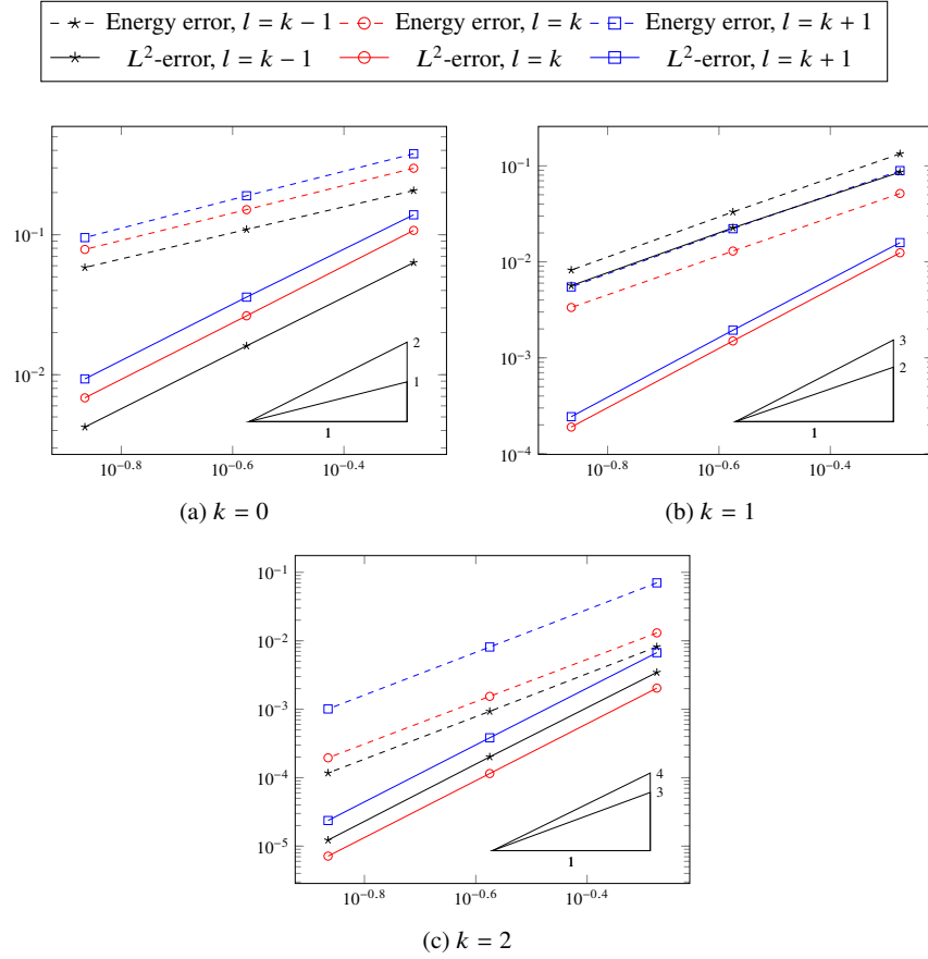
Fig. 5.6: Errors vs. h for the 3D test case in Section 5.1.8.2, simplicial meshes. Energy error refers to \|u_h - I_h^{k,\ell} u\|_{1,h} , L^2 -error refers to \|u_h - \pi_h^{0,\ell} u\| .
