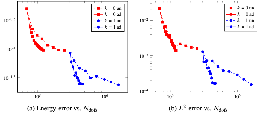
Fig. 4.4: Error vs. N_{\text{dofs}} for the test case of Section 4.1.3.2 and comparison with uniformly coarsened meshes.
