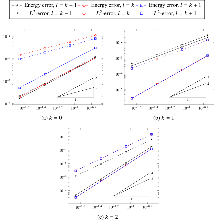
Fig. 5.4: Errors vs. h for the 2D test case in Section 5.1.8.1, locally refined Cartesian meshes. Energy error refers to \|\underline{u}_h - \underline{I}_h^{k,\ell} u\|_{1,h} , L^2 -error refers to \|u_h - \pi_h^{0,\ell} u\| .
