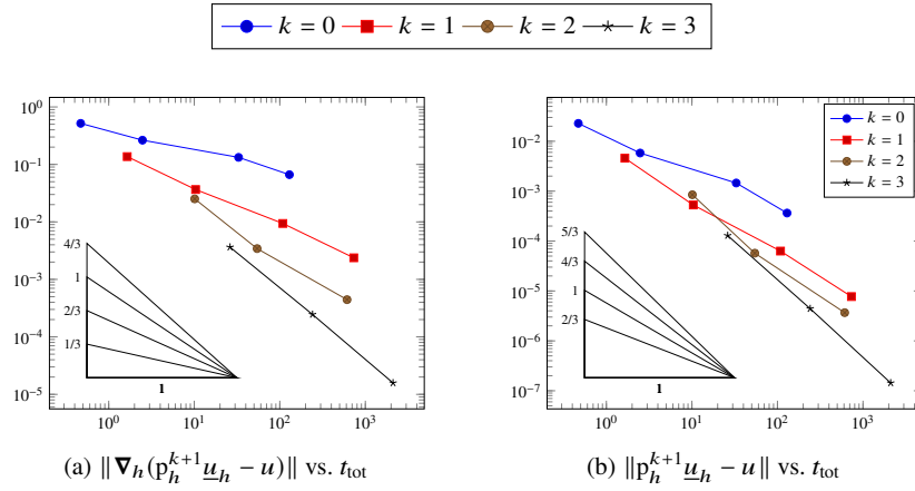
Fig. 2.5: Error vs. total computational time for the test case of Section 2.5.2. The reference slopes refer to the optimal scaling for each polynomial degree k \in \{0, \dots, 3\} .
