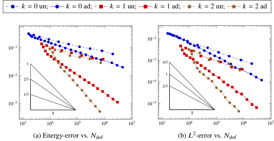
Fig. 4.1: Error vs. N_{\text{dof}} for the test case of Section 4.1.3.1. The triangles represent reference slopes corresponding to the optimal convergence rates.
