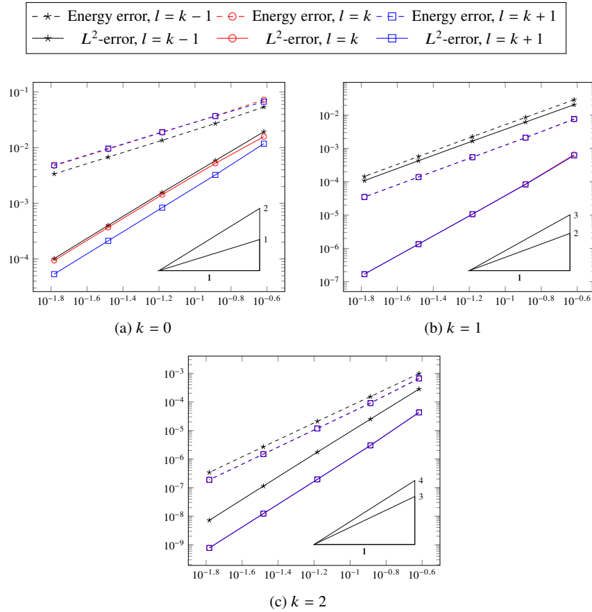
Fig. 5.3: Errors vs. h for the 2D test case in Section 5.1.8.1, hexagonal meshes. Energy error refers to \|u_h - I_h^{k,\ell} u\|_{1,h} , L^2 -error refers to \|u_h - \pi_h^{0,\ell} u\| .
