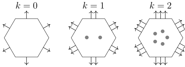
Fig. 5.8: Discrete unknowns in \underline{\boldsymbol{\Sigma}}_T^k for k \in \{0, 1, 2\} .
