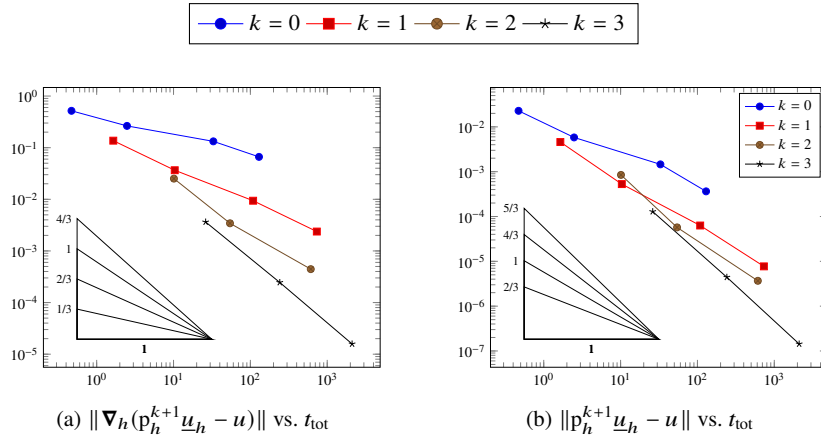
Fig. 2.5: Error vs. total computational time (in seconds) for the test case of Section 2.5.2. The reference slopes refer to the optimal scaling for each polynomial degree k \in \{0, \dots, 3\} .
