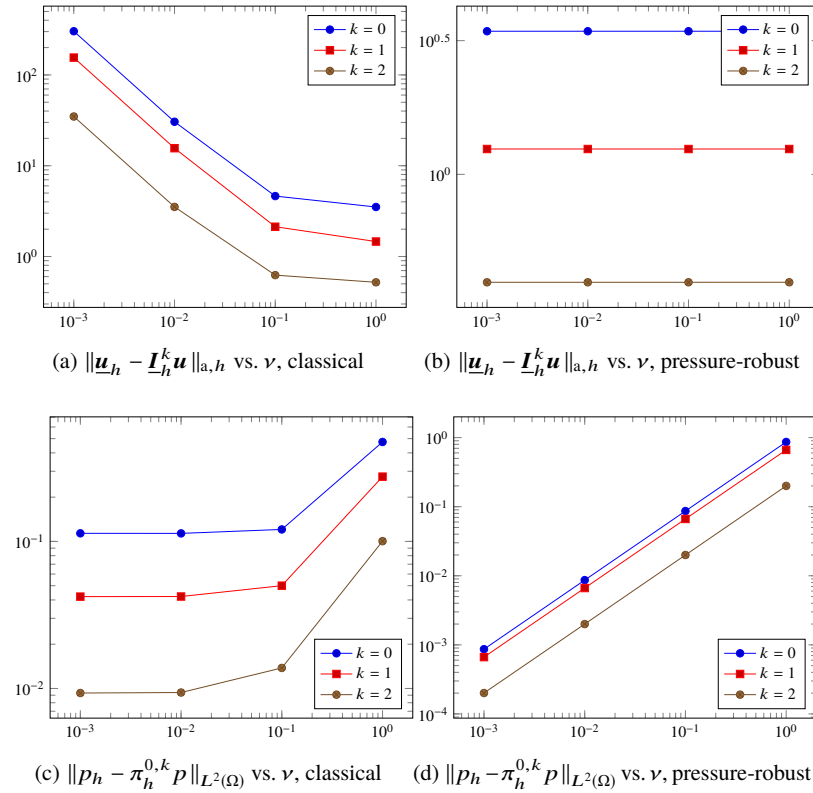
Fig. 8.3: Results for the numerical example of Section 8.6.5.1.
