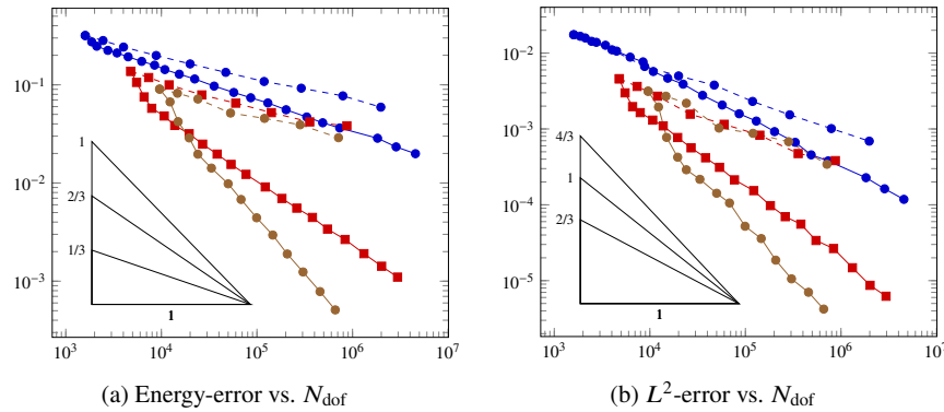
Fig. 4.1: Error vs. N_{\text{dof}} for the test case of Section 4.1.3.1. The triangles represent reference slopes corresponding to the optimal convergence rates. “un”= uniformly refined meshes, “ad”= adaptively refined meshes.
