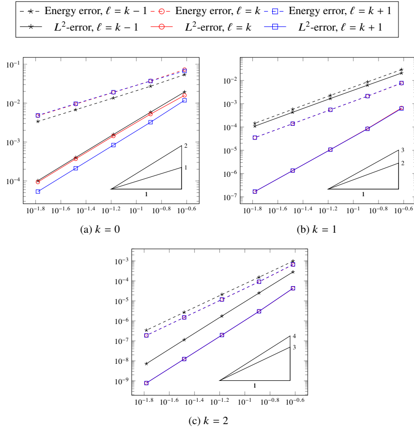
Fig. 5.3: Errors vs. h for the 2D test case in Section 5.1.8.1, hexagonal meshes. Energy error refers to \|u_h - \hat{u}_h\|_{1,h} , L^2 -error refers to \|u_h - \hat{u}_h\| , where \hat{u}_h = I_h^{k,\ell} u .
