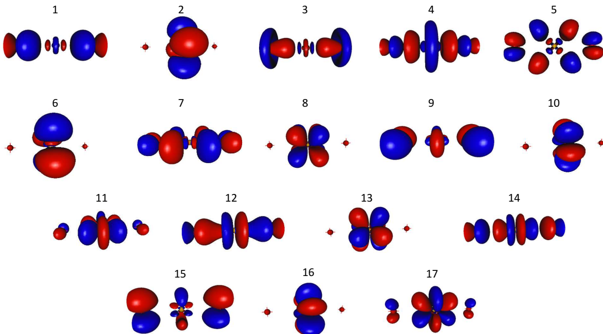
Figure 2: Molecular orbitals of \text{PuO}_2(\text{OH})_2 at CASSCF level. Isosurface = 0.05 au; Distances: Pu-OH = 2.103 Å, Pu-O = 1.742 Å; Angles: O-Pu-OH = 92.15°; HO-Pu-OH = 105.68°; O-Pu-O = 174.29°.
