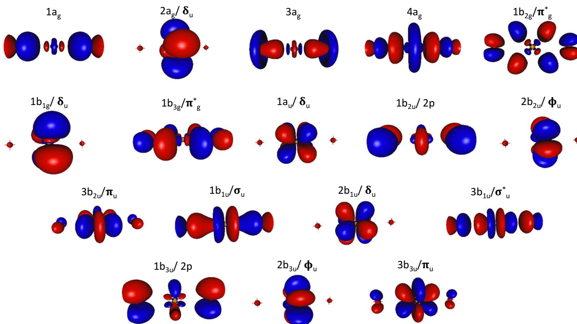
Figure 3: Molecular orbitals of \text{PuO}_2 at the CASSCF level; r(\text{Pu}-\text{O})=1.808 Å; Isosurface = 0.05 au.
