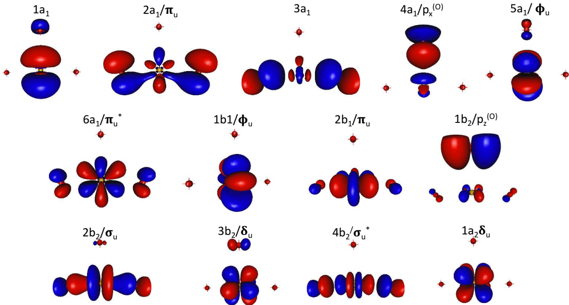
Figure 1: Active CASSCF orbitals of PuO 3 at the CASSCF level; Isosurface = 0.05 au; Distances: Pu-O(PuO 2 2+ subunit) = 1.767 Å; Pu-O axial = 1.934 Å; angle (O-Pu-O axial ) = 93.86°
