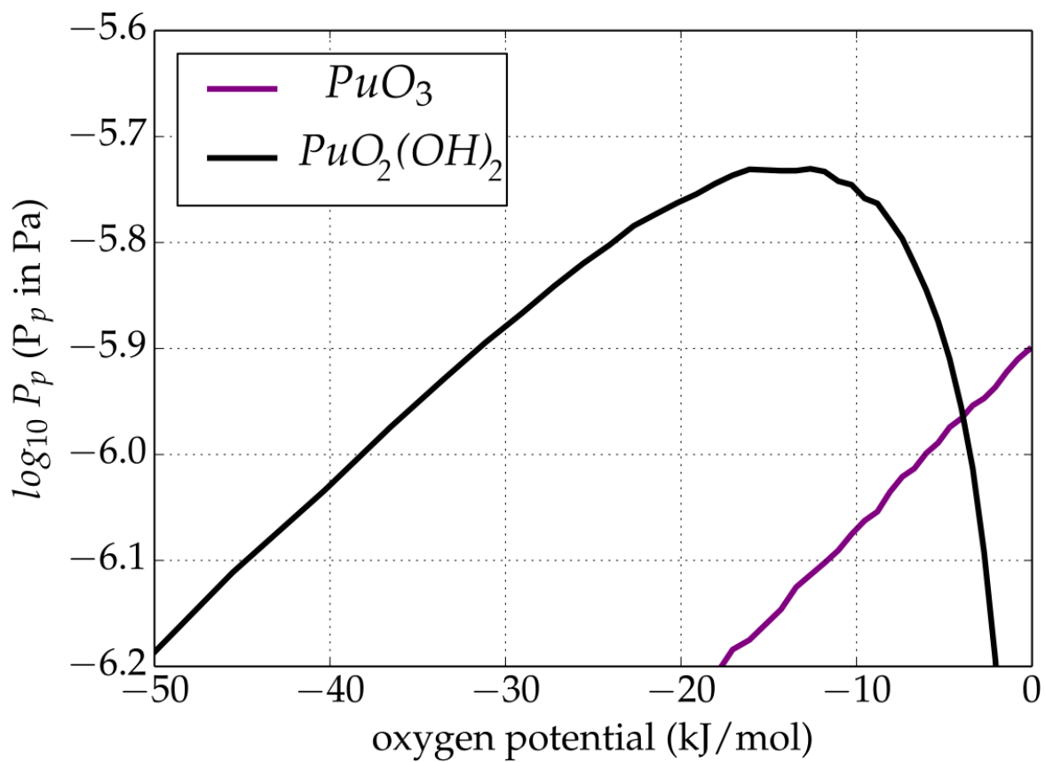
Figure 5: Focus on the partial pressures of plutonium species at 1500 K versus the chemical potential of oxygen under standard pressure conditions for the Pu-O-H system.
