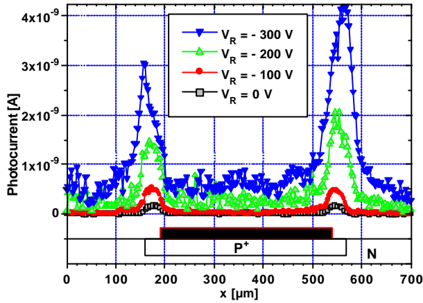
Fig. 3: OBIC measurements performed on a D1 diode without JTE at \lambda = 363.8 nm with P_{opt} = 2 W cm -2 for different reverse voltages.
