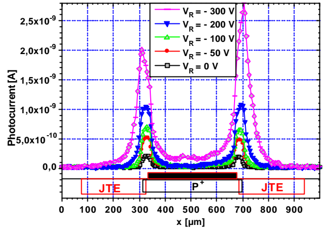
Fig. 4: OBIC measurements performed on a D2 diode with JTE at \lambda = 363.8 nm with P_{opt} = 2 W cm -2 for different reverse voltages.
