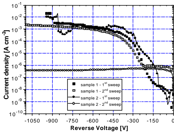
Fig. 1: Reverse electrical characteristics of diodes with JTE (D2), measured at 300 K in the air. Two bias sweeps are presented for each diode. The order of appearance in the legend corresponds to the chronological order of I-V measurement performed on each diode.
