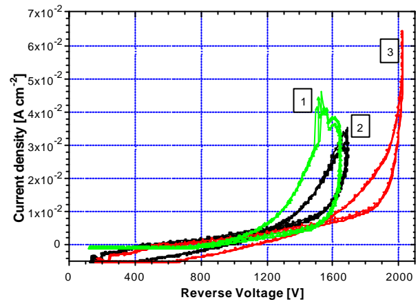
Fig. 2: Reverse electrical characteristics of diodes with JTE, measured at 300 K in the \text{SF}_6 ambient using a Tektronix 370A curve tracer. Three bias sweeps are presented for this diode and are numbered in the order of measurement.
