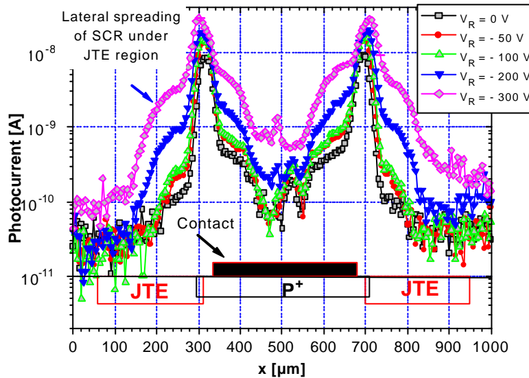
Fig. 5: OBIC measurements performed on a D2 diode with JTE at \lambda = 300 nm with P_{opt} = 2 W cm -2 for different reverse voltages.
