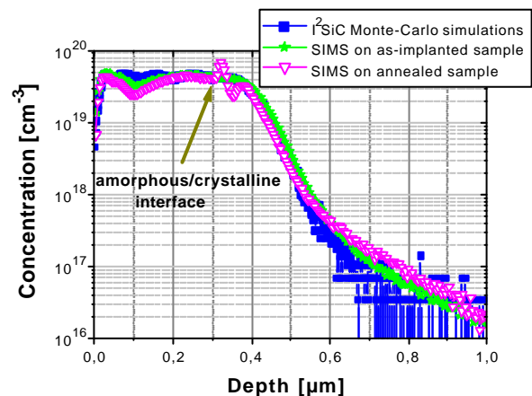
Fig. 3: SIMS analyses in as-implanted and 1700°C during 30 min annealed 6H-SiC samples, compared to ^6\text{SiC} Monte-Carlo simulation [3]
