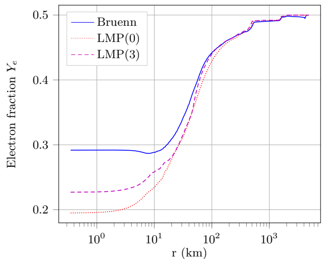
FIG. 3. (color online) Radial profiles of the electron fraction at bounce employing the three different EC rate prescriptions.
