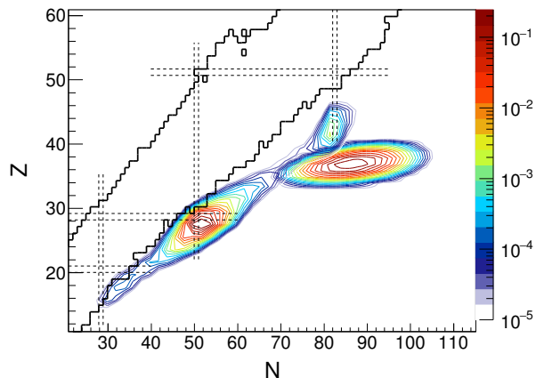
FIG. 9. (color online) Distribution of nuclei (N, Z) for a chosen thermodynamic condition during the collapse before trapping: T = 1 MeV; \rho_B = 6.02 \times 10^{11} g cm ^{-3} ; Y_e = 0.27 . Contour lines correspond to the cluster normalized probabilities (red to blue, more to less probable) for the original LS model (oval-shaped contour) and for the HFB-24 nuclear mass model. See text for details.
