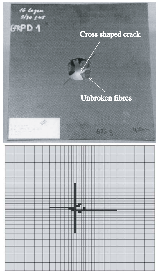
Figure 9 : Fully damaged zone after impact - experimental carbon-fiber / epoxy-resin on the left - numerical glass-fiber / epoxy-resin on the right
