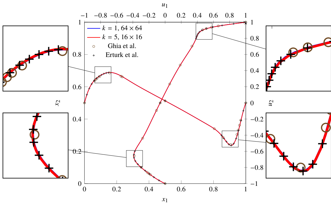
Figure 1: Two-dimensional lid-driven cavity flow, horizontal component u_1 of the velocity along the vertical centerline x_1 = \frac{1}{2} and the vertical component u_2 of the velocity along the horizontal centerline x_2 = \frac{1}{2} for Re = 1,000 .
