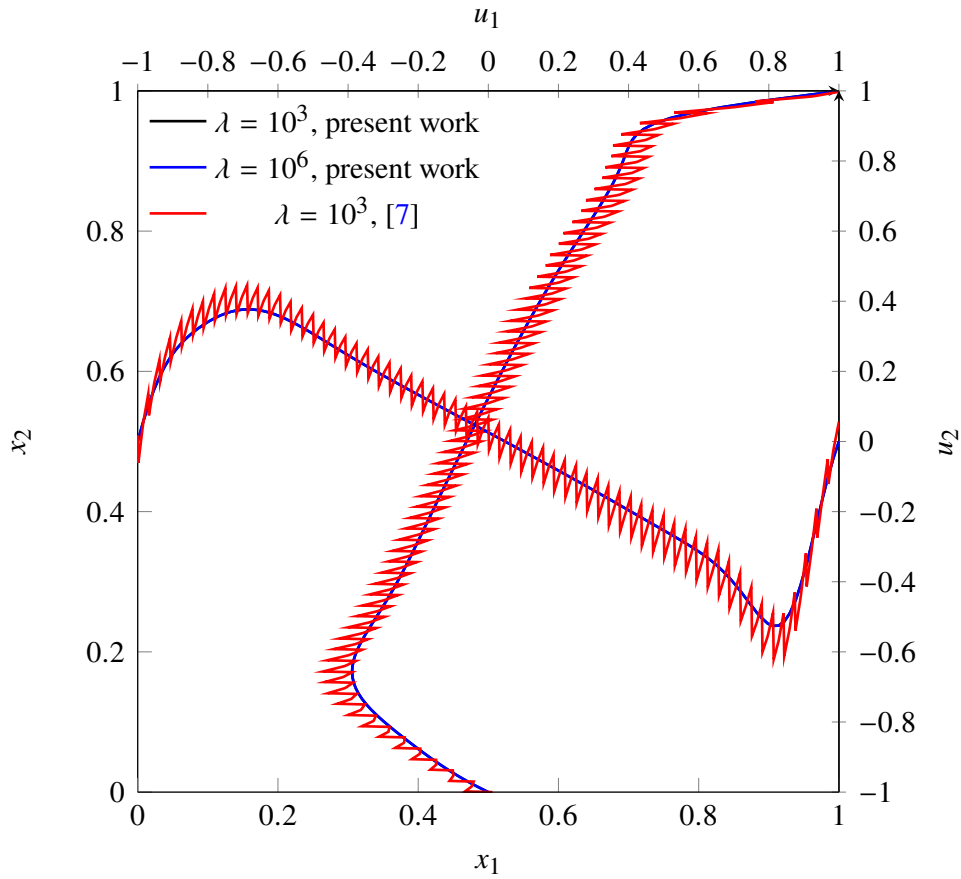
Figure 3: Two-dimensional lid-driven cavity flow with irrotational force \mathbf{f} = \lambda \nabla \psi with \lambda \in \{10^3, 10^6\} . Comparison between the present method and the original HHO formulation of [7]. The plot represents the horizontal component u_1 of the velocity along the vertical centerline x_1 = \frac{1}{2} and the vertical component u_2 of the velocity along the horizontal centerline x_2 = \frac{1}{2} for \text{Re} = 1,000 .
