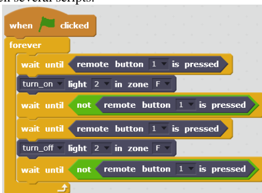
Fig. 7. Scratch 2.0 script for the light control
