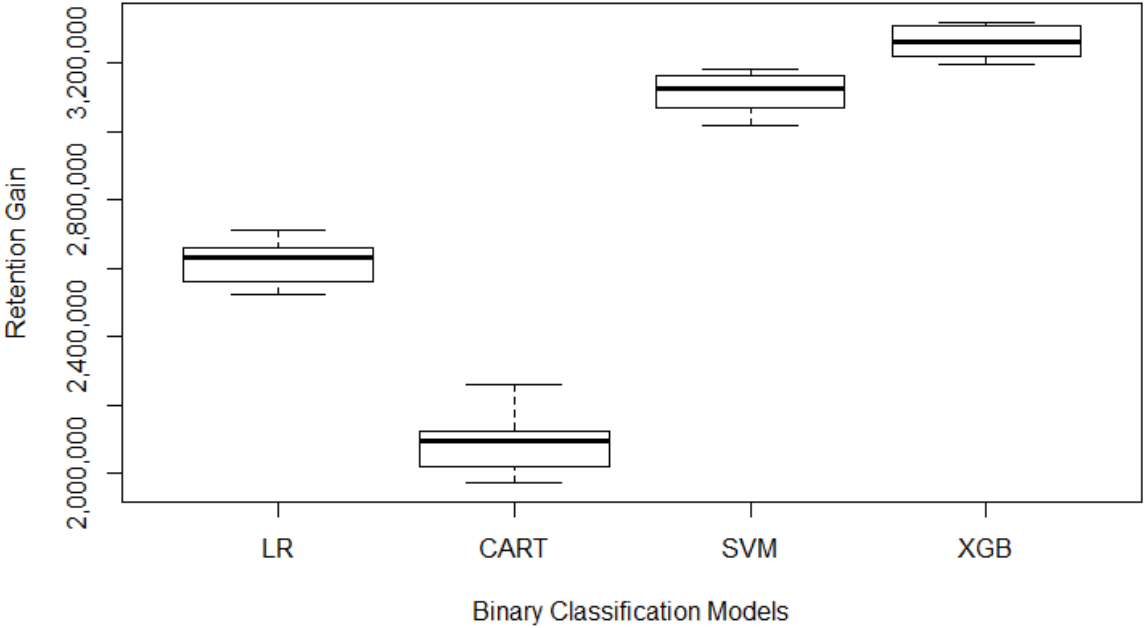
Figure 3: Box Plot of Retention Gains with the Moderate Strategy
