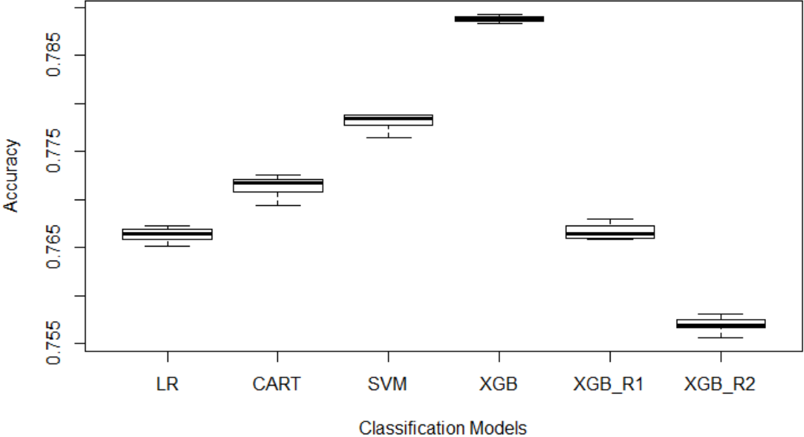
Figure 4: Box Plot of Cross-Validated Accuracy
