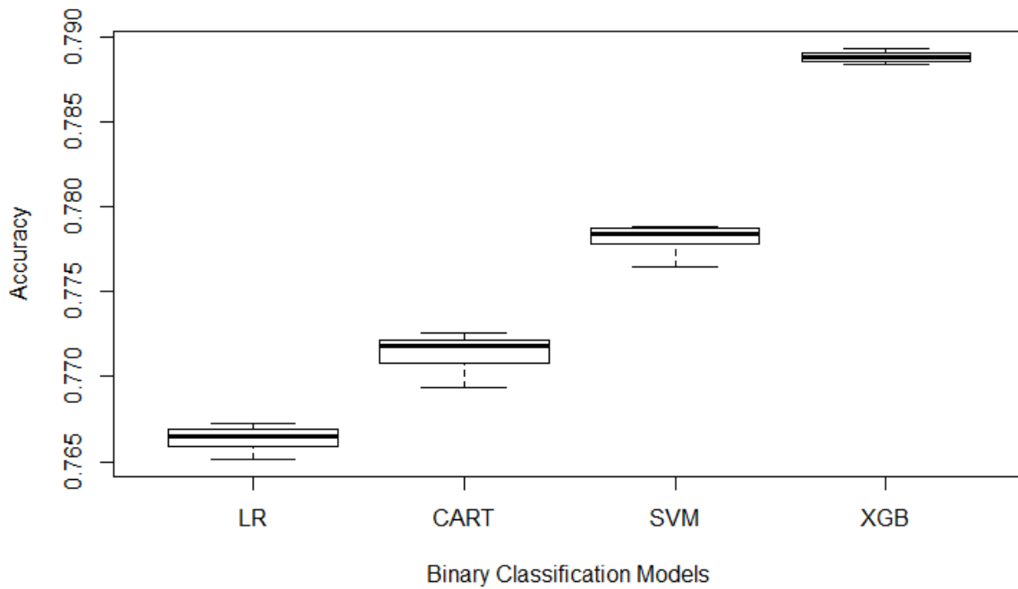
Figure 1: Box Plot of Statistic Accuracies
