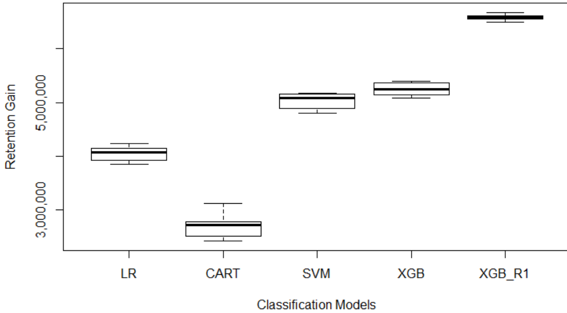
Figure 5: Box Plot of Retention Gains the Aggressive Strategy
