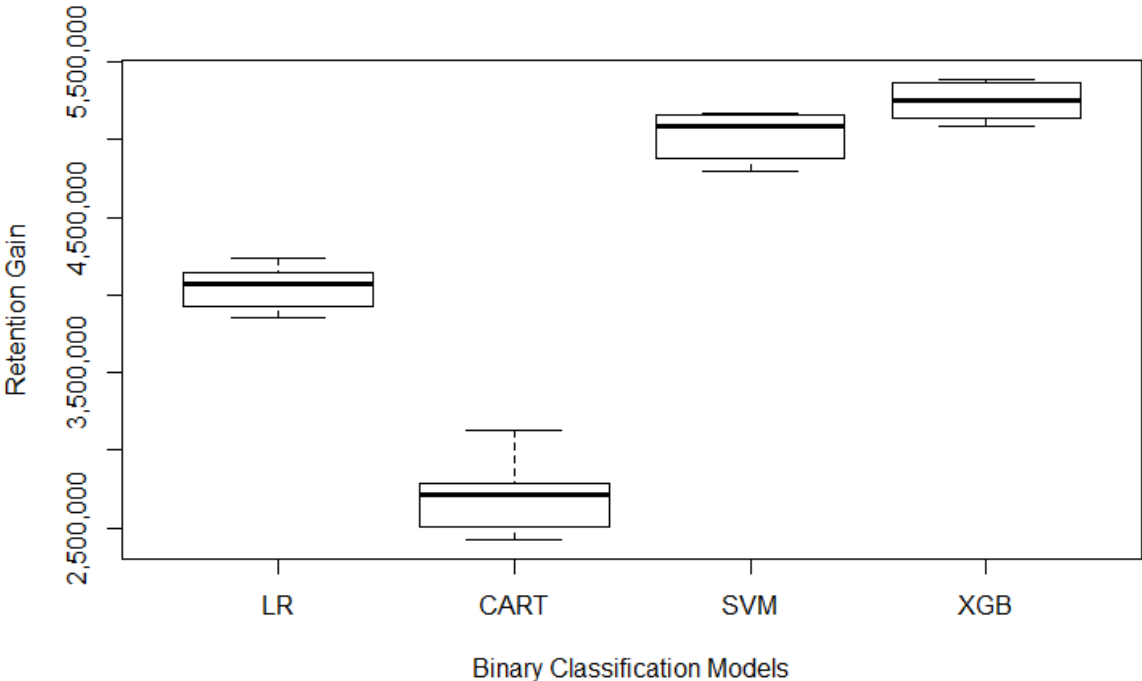
Figure 2: Box Plot of Retention Gains with the Aggressive Strategy
