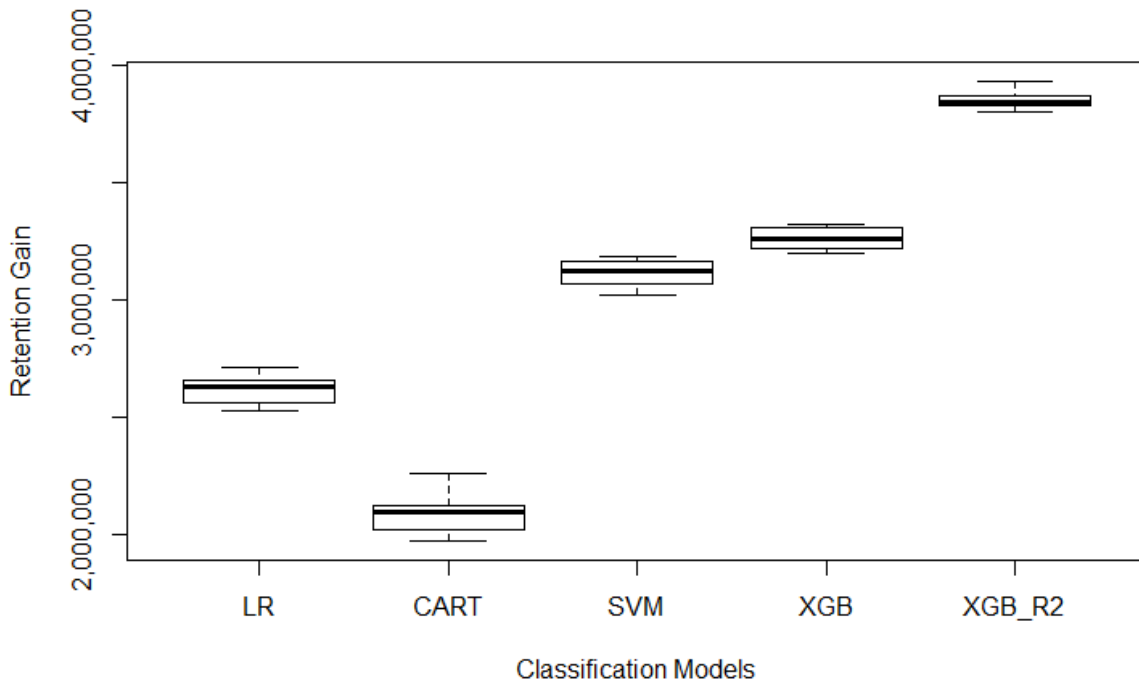
Figure 6: Box Plot of Retention Gains the Moderate Strategy
