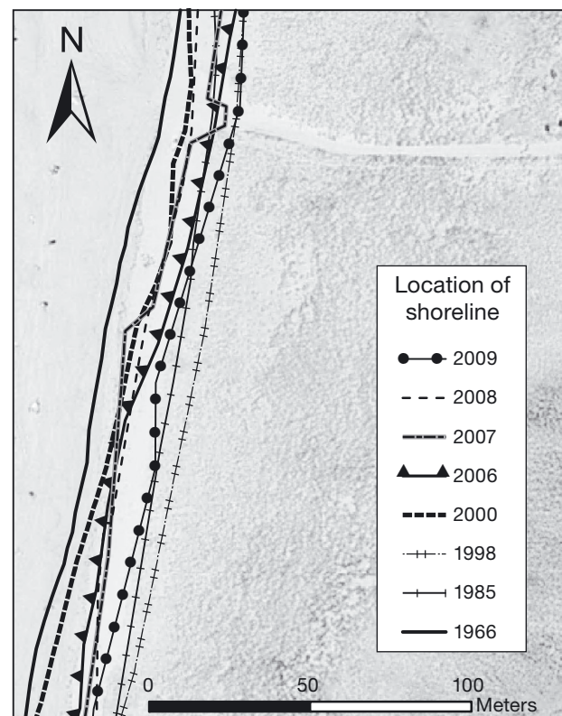
Fig. 4. Shoreline position from 1966 to 2009 at Truc Vert beach. The shoreline shown is the high water mark, i.e. the boundary between dune and beach. Background image — projection system: RGF 93 / Lambert 93; Copyright: Orthophoto 2009 IGN (GIP ATGeRI); dataset: BRGM Aquitaine Coast Observatory (40 cm resolution)
