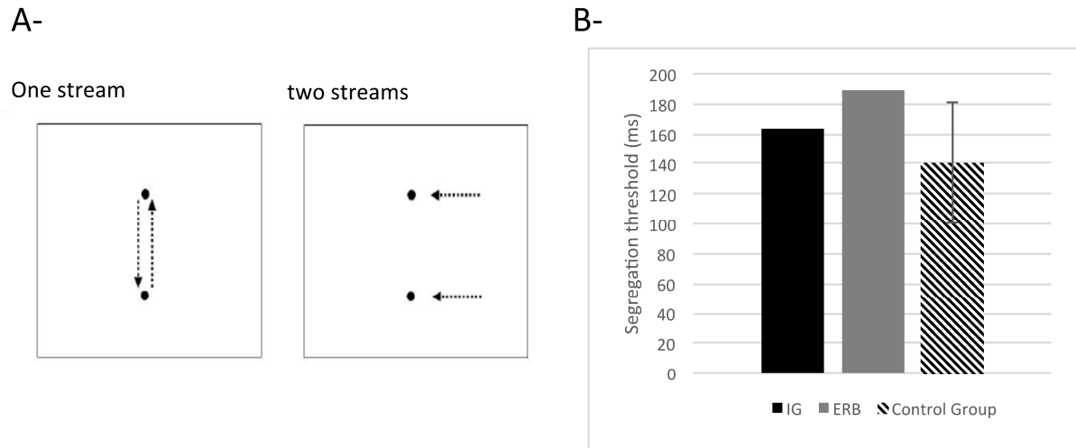
7 8 Figure 6: (A) Schematic representation of the visual stream segregation procedure 9 (Experiment 3). The dotted arrows symbolise the one-stream (longer SOAs) or two stream 10 (shorter SOAs) conditions. (B) Segregation threshold for IG (black), ERB (grey) and the 11 controls (hatch) in milliseconds. The standard error bars are provided for the control group.
