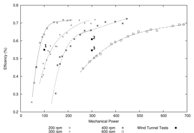
Fig 4. Generator performance behavior in relation to the mechanical power for different rotational speeds. The points represent experimental data and the curves are fitted laws.
