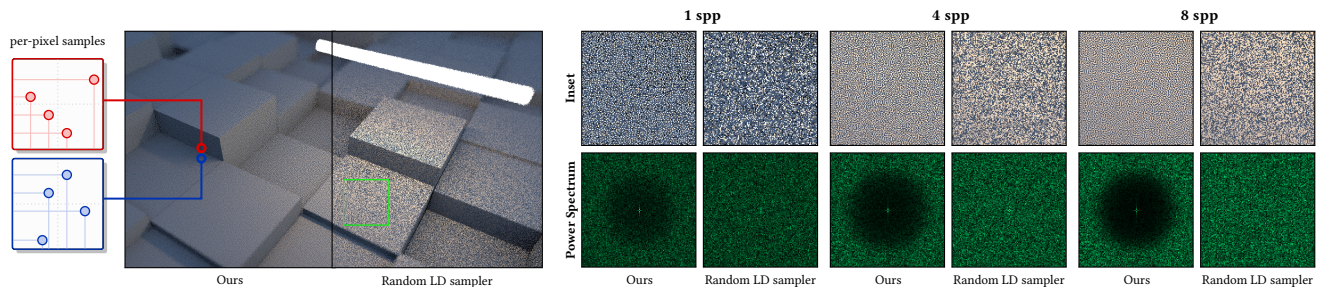
Figure 1: Our sampler distributes per-pixel sample sets such that their Monte Carlo errors is a blue noise in screen space. This increases the visual quality of the renders in contrast to randomly distributing the sample sets.
