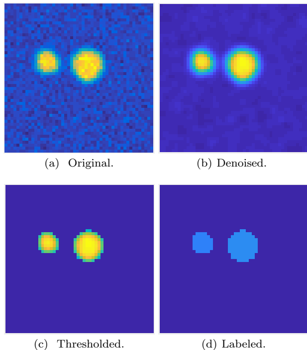
Fig. 3.1 Particular of the frame of Figure 2.1(c). (a): a region of interest with two separated particles. (b): result of the Gaussian filtering. The noise is reduced, but the edges are blurred. (c): thresholding via the Otsu method. (d): labeling procedure, where different colors mean different labels. The order of labeling does not influence the final result.
