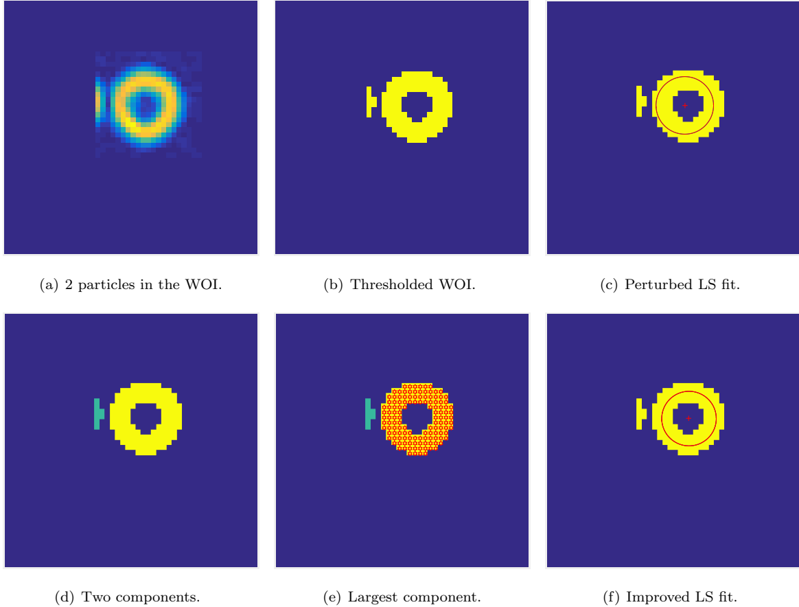
Figure 4: Upper panels: when two (or more) particles are very close but still separated, selecting a large WOI may lead to include some undesired pixels in the LS fit, resulting into a perturbed result. Bottom panels: searching inside the WOI for all connected components avoids the problem depicted in upper panels. If the particles are close but disconnected, one can easily isolate the largest component which is related to the particle, and hence a reliable LS fit can be reached.
