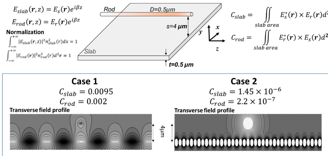
Figure 14. Top: Schematics of an optical coupling between a cylindrical dielectric rod and a semi-infinite dielectric slab. The rod has a diameter of 0.5 \mu\text{m} and a refractive index n_{rod} = 1.45 , the slab thickness is set to 0.5 \mu\text{m} , and the distance between the rod and the slab to 4 \mu\text{m} . The operating wavelength \lambda = 1.55 \mu\text{m} for two cases. Case 1: the slab index is n_{slab} = 1.1 . Case 2: n_{slab} = 1.45 . Bottom: Calculated electric transverse field profile and the overlap integrals for the two cases.
