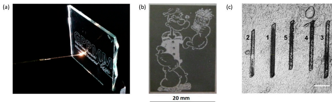
Figure 25. Illustrations of different applications of HCPCF fiber laser beam delivery, with (a) glass engraving (reprinted with permission from Reference [17], OSA, 2013), (b) titanium micromachining (reprinted with permission from Reference [107], OSA, 2015), and (c) tissue surface ablation (reprinted with permission from Reference [111], OSA, 2016).
