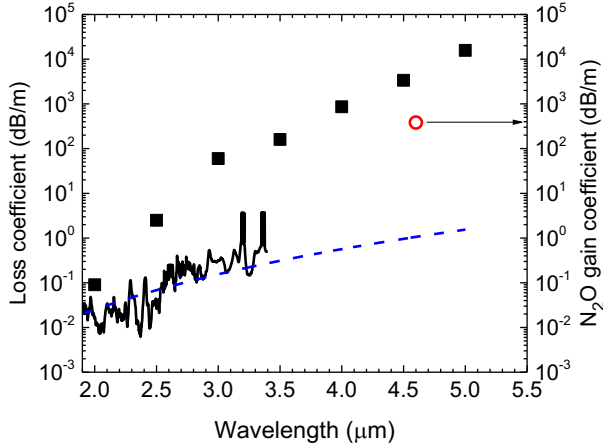
Fig.2. Loss coefficient \kappa_F versus wavelength for bulk fused silica (squares, data from Heraeus Suprasil 300 [17]), measured loss in the HCPCF used for our HOFGLAS (solid line) and extrapolation of the loss to \lambda = 5 \mu\text{m} using the scaling law \alpha_{\text{wg}} \propto \lambda^{4.3} [18] (dashed line). The open circle corresponds to the calculated gain coefficient at 4.6 \mu\text{m} , see text.
