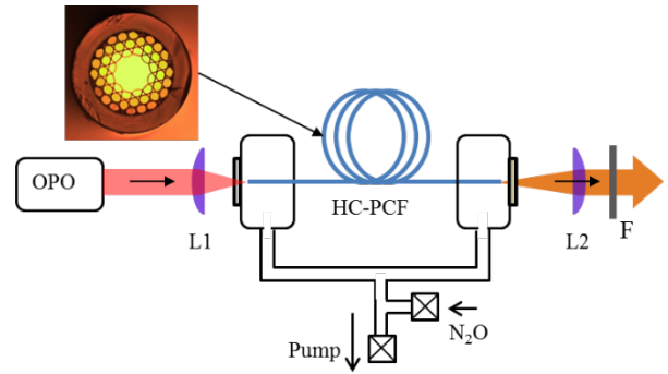
Fig.3. Experimental setup of the 4.6- \mu\text{m} pulsed \text{N}_2\text{O} laser. The inset shows the cross section of the 45-cm long fiber. The pump was an 8-ns pulse at 1.517 \mu\text{m} from an OPO. To control the pressure the two ends of the fiber were housed in small chambers. “F” denotes a long pass germanium filter used to block residual pump radiation.
