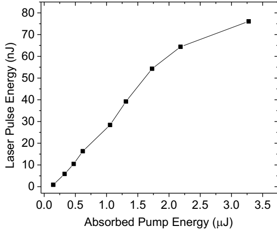
Fig.6. Laser pulse energy as a function of absorbed pump pulse energy for a 45-cm long fiber filled with 80 Torr N_2O gas.
