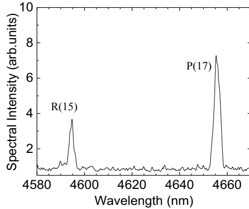
Fig.4. Measured spectrum of the \text{N}_2\text{O} laser. Details of the lines are not resolved. p = 80 Torr, absorbed pump energy E_{\text{abs}} = 1.3 \mu\text{J} .
