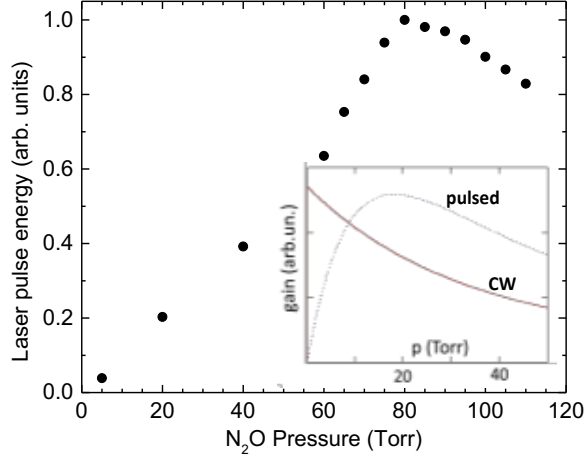
Fig.5. Measured laser output as a function of N_2O pressure for 70 \mu J of pump energy coupled into fiber. The inset shows the calculated gain coefficient g_{32}(p) , see text.
