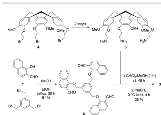
Scheme 2 Synthesis of the fluorescent hemicryptophane host 3.
