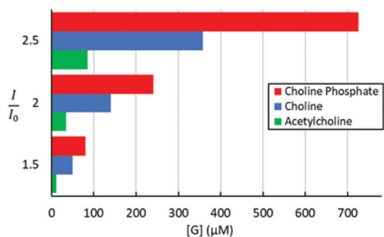
Fig. 3 Increase by 50%, 100% and 150% of the normalized intensity of a 5 \mu\text{M} solution of 3 in DMSO + 2% \text{H}_2\text{O} with respect to the concentration of the corresponding added guest at 298 K (counterion \text{Cl}^- for ACh, Ch and \text{Cl}^- and \text{Ca}^{2+} for choline phosphate).
