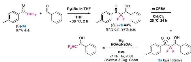
Scheme 4. Synthesis of \beta -hydroxysulfoxide ( S_2 )-7a from enantiopure (S)-difluoromethyl p -tolyl sulfoxide (S)-3a, oxidation and and stereo-retentive desulfonylation
