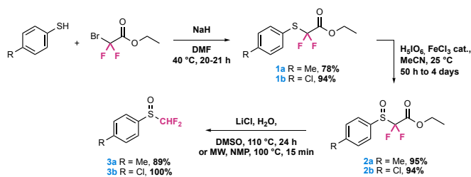
Scheme 1. Synthesis of racemic \alpha,\alpha -difluoromethyl sulfoxides 3a and 3b
