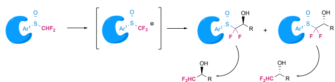
Figure 1. Methodology to access to \alpha,\alpha -difluoromethyl alcohols by means of an enantiopure \alpha,\alpha -difluoromethyl sulfoxide
