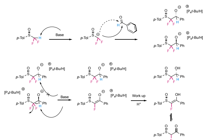
Scheme 3. Proposed mechanism to explain the good diastereoselectivities
