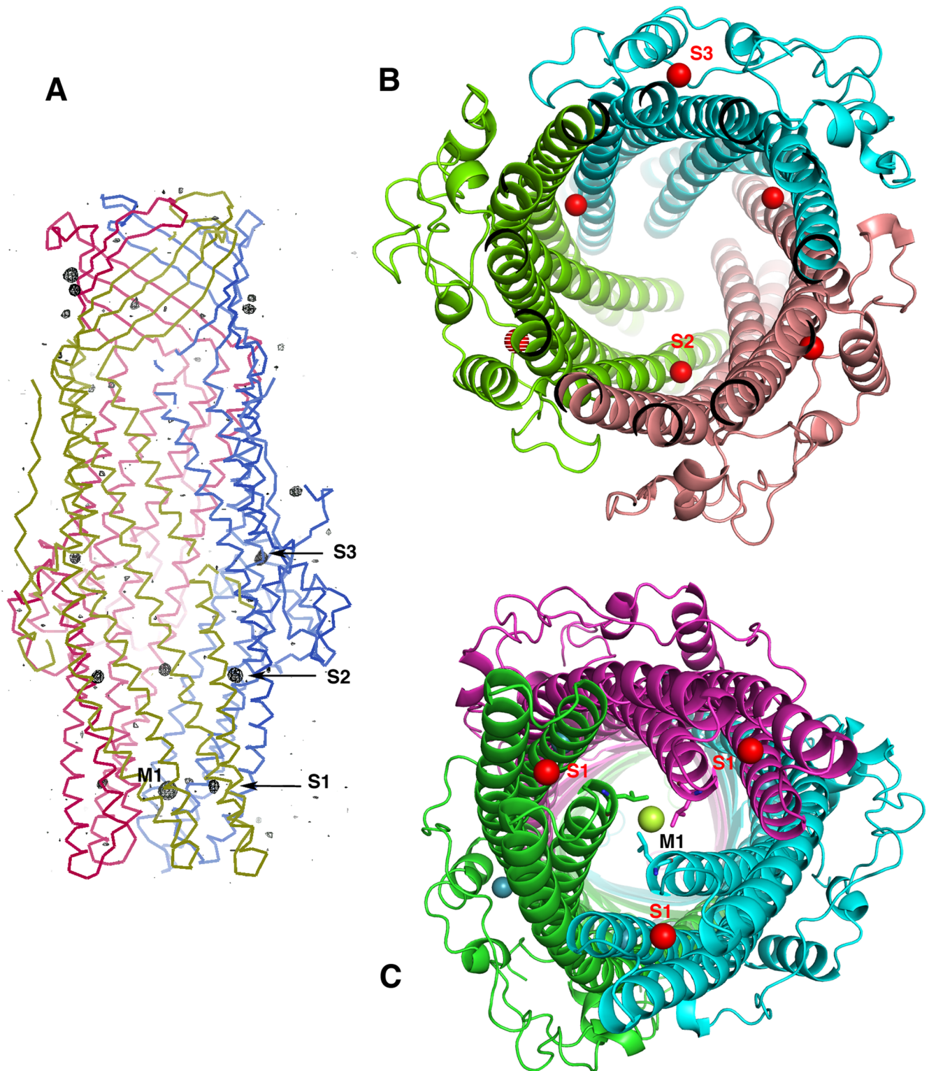
Fig 2. A: The anomalous map—in black tracing and contour at 3.5 \sigma .—superimposed to the C \alpha tracing of the OprN structure. The three S1 to S3 sites are labelled. On top of the structure, outside of the \beta -barrel, four more xenon atoms are present around the \beta -barrel domain, in a fully hydrophobic environment. B: (view from the extra cellular side) The two inter and intra-subunit S2 and S3 sites in the helical \alpha -domain (xenon as red spheres) viewed along the central channel of the trimer. C: (view from the periplasmic side) The M1 site locked by the three equivalent Leu 405, viewed along the central channel of OprN-Xe structure at the periplasmic entrance. The S1 secondary sites are located at the same level of the main M1 site in a plane perpendicular to the tunnel. S1 xenon atoms are in red, M1 xenon in lime green. The three monomers building the cylindrical scaffold are in three different colours.
